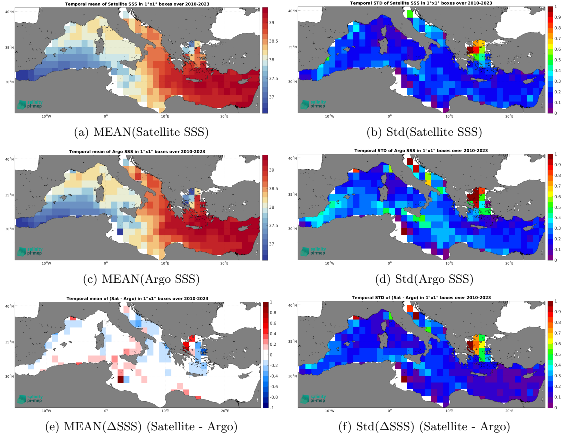
Figure 6: Temporal mean (left) and Std (right) of SSS from SMOS SSS L4 v1 - Weekly (CMEMS-CNR) (top), Argo (middle), and of \Delta\text{SSS} (Satellite - Argo). Only match-up pairs are used to generate these maps.
