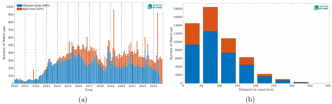
Figure 1: Number of match-ups between Argo and SMOS SSS L4 v1 - Weekly (CMEMS-CNR) SSS as a function of time (a) and as function of the distance to coast (b) over the Mediterranean Sea Pi-MEP region and for the full satellite product period.
