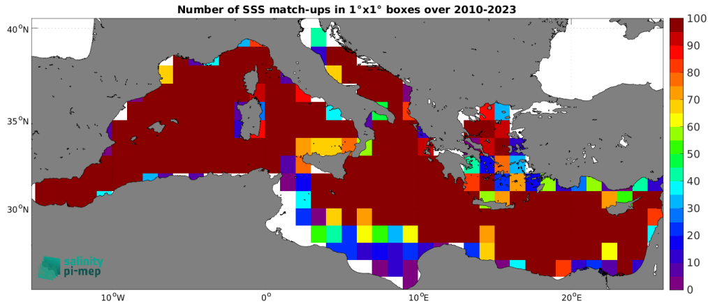
Figure 4: Number of SSS match-ups between Argo SSS and the SMOS SSS L4 v1 - Weekly (CMEMS-CNR) SSS product for the Mediterranean Sea Pi-MEP region over 1^\circ \times 1^\circ boxes and for the full satellite product period.
