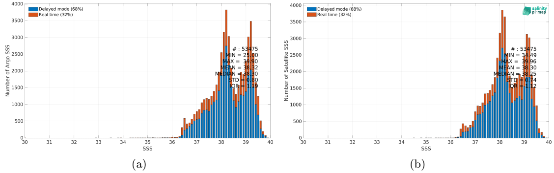
Figure 2: Histograms of SSS from Argo (a) and SMOS SSS L4 v1 - Weekly (CMEMS-CNR) (b) considering all match-up pairs per bins of 0.1 over the Mediterranean Sea Pi-MEP region and for the full satellite product period.
