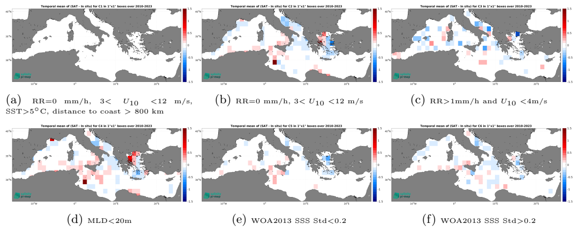
Figure 12: Temporal mean gridded over spatial boxes of size 1^\circ \times 1^\circ of \Delta SSS (SMOS SSS L4 v1 - Weekly (CMEMS-CNR) - Argo) for 6 different subdatasets corresponding to:RR=0 mm/h, 3 < U_{10} < 12 m/s, SST >5^\circ\text{C} , distance to coast > 800 km (a), RR=0 mm/h, 3 < U_{10} < 12 m/s (b), RR >1 mm/h and U_{10} < 4 m/s (c),MLD <20 m (d),WOA2013 SSS Std <0.2 (e),WOA2013 SSS Std >0.2 (f).
