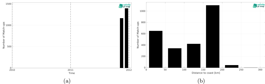
Figure 2: Number of match-ups between TSG (SAMOS) and SMOS SSS L4 v1 - Monthly (CMEMS-CNR) SSS as a function of time (a) and as function of the distance to coast (b) over the Mediterranean Sea Pi-MEP region and for the full satellite product period.
