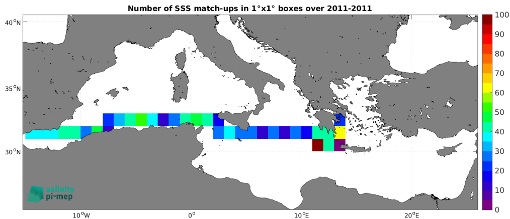
Figure 5: Number of SSS match-ups between TSG (SAMOS) SSS and the SMOS SSS L4 v1 - Monthly (CMEMS-CNR) SSS product for the Mediterranean Sea Pi-MEP region over 1^\circ \times 1^\circ boxes and for the full satellite product period.
