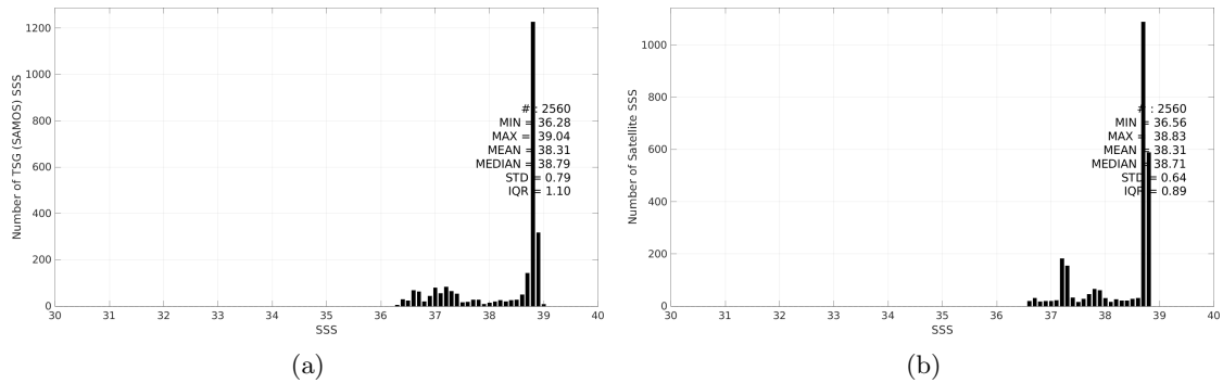
Figure 3: Histograms of SSS from TSG (SAMOS) (a) and SMOS SSS L4 v1 - Monthly (CMEMS-CNR) (b) considering all match-up pairs per bins of 0.1 over the Mediterranean Sea Pi-MEP region and for the full satellite product period.
