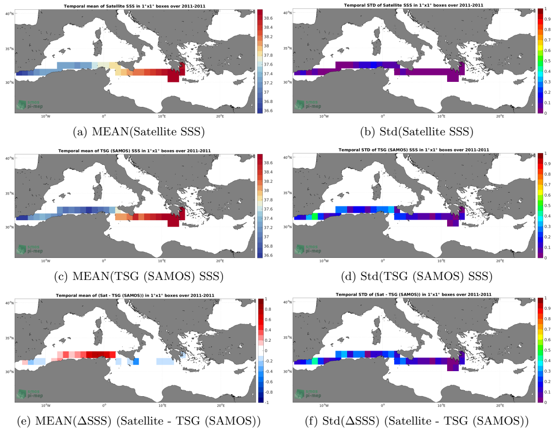
Figure 6: Temporal mean (left) and Std (right) of SSS from SMOS SSS L4 v1 - Monthly (CMEMS-CNR) (top), TSG (SAMOS) ( in situ ) dataset (middle), and of \Delta SSS (Satellite - TSG (SAMOS)). Only match-up pairs are used to generate these maps.
