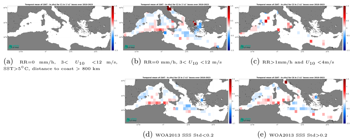
Figure 14: Temporal mean gridded over spatial boxes of size 1^\circ \times 1^\circ of \Delta\text{SSS} (SMOS SSS L4 v1 - Monthly (CMEMS-CNR) - TSG (LEGOS-DM)) for 5 different subdatasets corresponding to:RR=0 mm/h, 3 < U_{10} < 12 m/s, SST>5°C, distance to coast > 800 km (a), RR=0 mm/h, 3 < U_{10} < 12 m/s (b), RR>1mm/h and U_{10} < 4 m/s (c), WOA2013 SSS Std<0.2 (d), WOA2013 SSS Std>0.2 (e).
