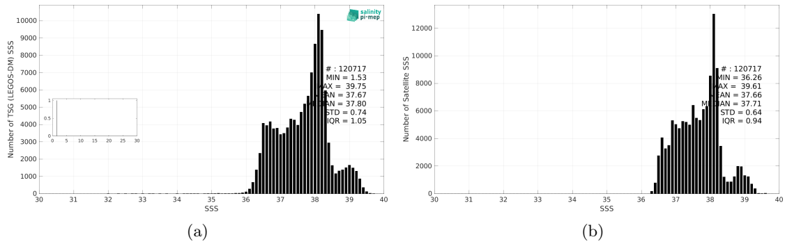
Figure 3: Histograms of SSS from TSG (LEGOS-DM) (a) and SMOS SSS L4 v1 - Monthly (CMEMS-CNR) (b) considering all match-up pairs per bins of 0.1 over the Mediterranean Sea Pi-MEP region and for the full satellite product period.
