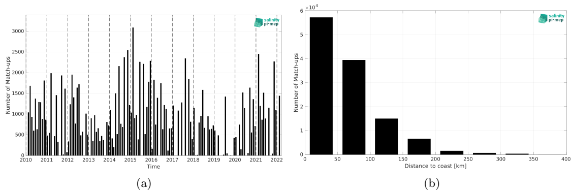
Figure 2: Number of match-ups between TSG (LEGOS-DM) and SMOS SSS L4 v1 - Monthly (CMEMS-CNR) SSS as a function of time (a) and as function of the distance to coast (b) over the Mediterranean Sea Pi-MEP region and for the full satellite product period.
