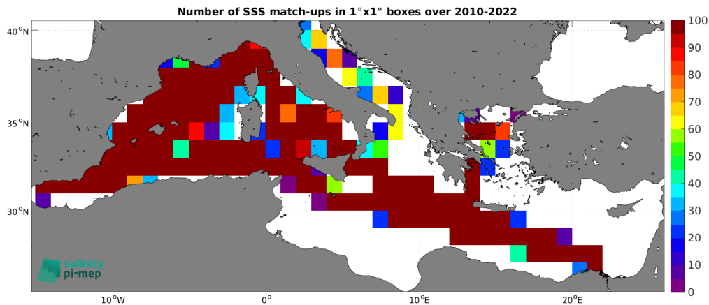
Figure 5: Number of SSS match-ups between TSG (LEGOS-DM) SSS and the SMOS SSS L4 v1 - Monthly (CMEMS-CNR) SSS product for the Mediterranean Sea Pi-MEP region over 1^\circ \times 1^\circ boxes and for the full satellite product period.
