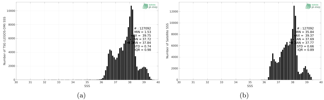
Figure 2: Histograms of SSS from TSG (LEGOS-DM) (a) and SMOS SSS L4 v1 - Monthly (CMEMS-CNR) (b) considering all match-up pairs per bins of 0.1 over the Mediterranean Sea Pi-MEP region and for the full satellite product period.
