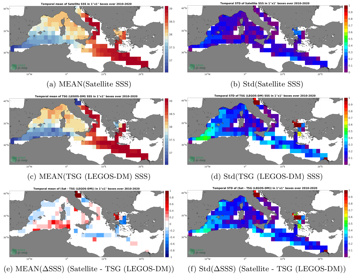
Figure 6: Temporal mean (left) and Std (right) of SSS from SMOS SSS L4 v1 - Monthly (CMEMS-CNR) (top), TSG (LEGOS-DM) (middle), and of \Delta SSS (Satellite - TSG (LEGOS-DM)). Only match-up pairs are used to generate these maps.
