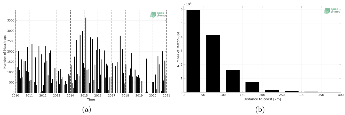
Figure 1: Number of match-ups between TSG (LEGOS-DM) and SMOS SSS L4 v1 - Monthly (CMEMS-CNR) SSS as a function of time (a) and as function of the distance to coast (b) over the Mediterranean Sea Pi-MEP region and for the full satellite product period.
