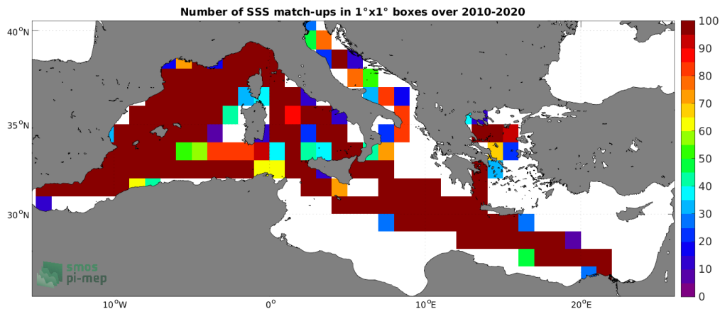
Figure 4: Number of SSS match-ups between TSG (LEGOS-DM) SSS and the SMOS SSS L4 v1 - Monthly (CMEMS-CNR) SSS product for the Mediterranean Sea Pi-MEP region over 1^\circ \times 1^\circ boxes and for the full satellite product period.
