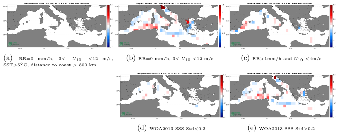
Figure 12: Temporal mean gridded over spatial boxes of size 1^\circ \times 1^\circ of \Delta SSS (SMOS SSS L4 v1 - Monthly (CMEMS-CNR) - TSG (LEGOS-DM)) for 5 different subdatasets corresponding to:RR=0 mm/h, 3 < U_{10} < 12 m/s, SST >5^\circ\text{C} , distance to coast > 800 km (a), RR=0 mm/h, 3 < U_{10} < 12 m/s (b), RR >1 mm/h and U_{10} < 4 m/s (c), WOA2013 SSS Std <0.2 (d), WOA2013 SSS Std >0.2 (e).
