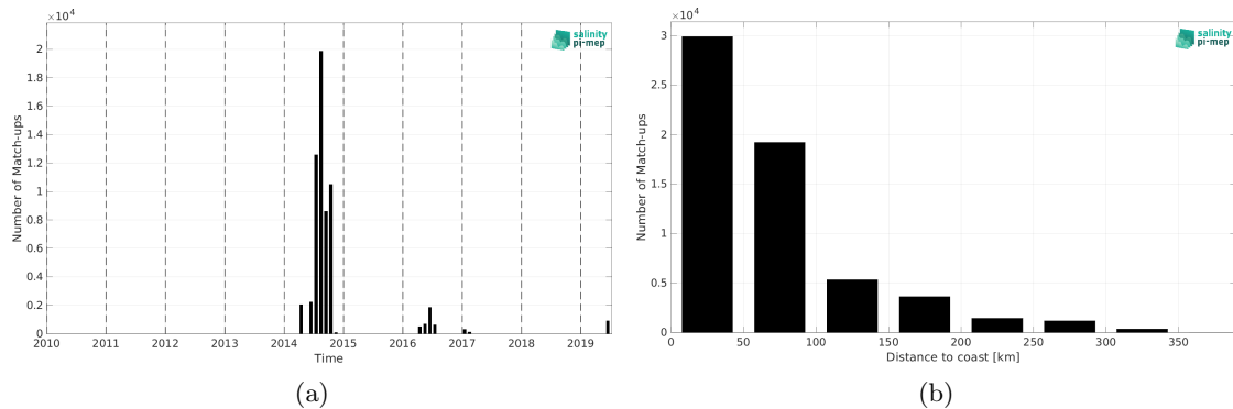
Figure 2: Number of match-ups between TSG (GOSUD-Sailing-ship) and SMOS SSS L4 v1 - Monthly (CMEMS-CNR) SSS as a function of time (a) and as function of the distance to coast (b) over the Mediterranean Sea Pi-MEP region and for the full satellite product period.
