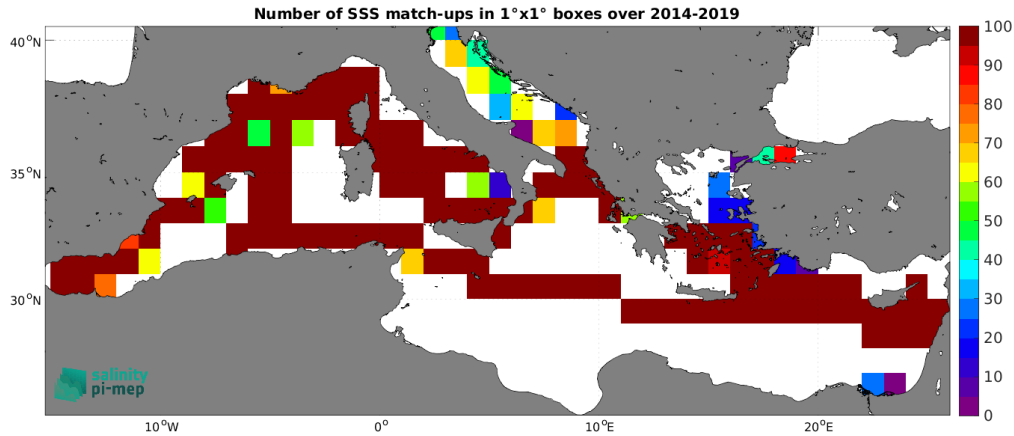
Figure 5: Number of SSS match-ups between TSG (GOSUD-Sailing-ship) SSS and the SMOS SSS L4 v1 - Monthly (CMEMS-CNR) SSS product for the Mediterranean Sea Pi-MEP region over 1^\circ \times 1^\circ boxes and for the full satellite product period.
