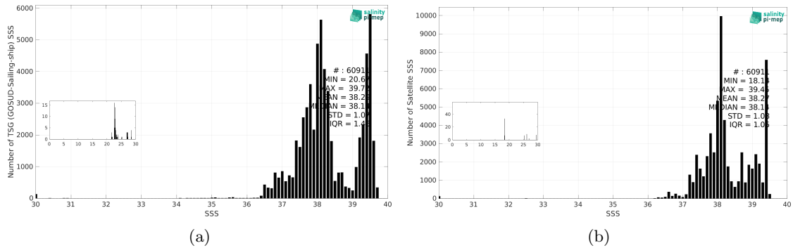
Figure 3: Histograms of SSS from TSG (GOSUD-Sailing-ship) (a) and SMOS SSS L4 v1 - Monthly (CMEMS-CNR) (b) considering all match-up pairs per bins of 0.1 over the Mediterranean Sea Pi-MEP region and for the full satellite product period.
