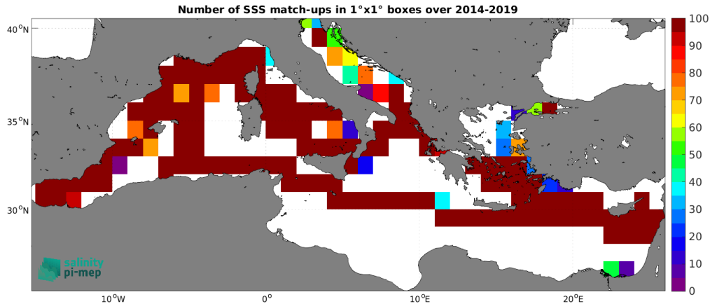
Figure 4: Number of SSS match-ups between TSG (GOSUD-Sailing-ship) SSS and the SMOS SSS L4 v1 - Monthly (CMEMS-CNR) SSS product for the Mediterranean Sea Pi-MEP region over 1°x1° boxes and for the full satellite product period.
