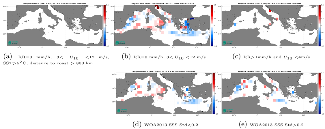
Figure 12: Temporal mean gridded over spatial boxes of size 1^\circ \times 1^\circ of \Delta\text{SSS} (SMOS SSS L4 v1 - Monthly (CMEMS-CNR) - TSG (GOSUD-Sailing-ship)) for 5 different subdatasets corresponding to:RR=0 mm/h, 3 < U_{10} < 12 m/s, SST >5^\circ\text{C} , distance to coast > 800 km (a), RR=0 mm/h, 3 < U_{10} < 12 m/s (b), RR >1 mm/h and U_{10} < 4 m/s (c), WOA2013 SSS Std <0.2 (d), WOA2013 SSS Std >0.2 (e).
