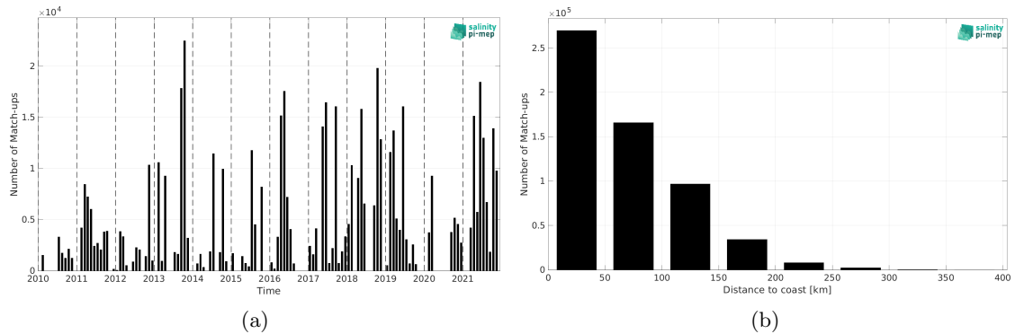
Figure 2: Number of match-ups between TSG (GOSUD-Research-vessel) and SMOS SSS L4 v1 - Monthly (CMEMS-CNR) SSS as a function of time (a) and as function of the distance to coast (b) over the Mediterranean Sea Pi-MEP region and for the full satellite product period.
