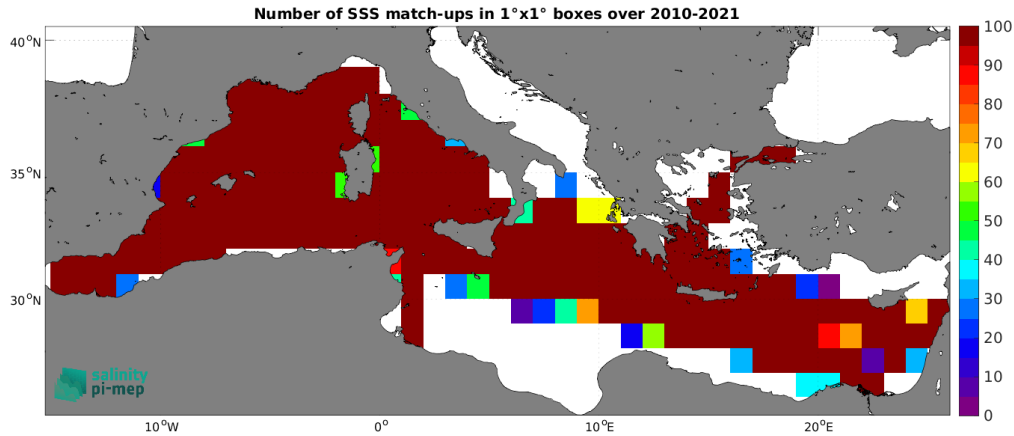
Figure 5: Number of SSS match-ups between TSG (GOSUD-Research-vessel) SSS and the SMOS SSS L4 v1 - Monthly (CMEMS-CNR) SSS product for the Mediterranean Sea Pi-MEP region over 1^\circ \times 1^\circ boxes and for the full satellite product period.
