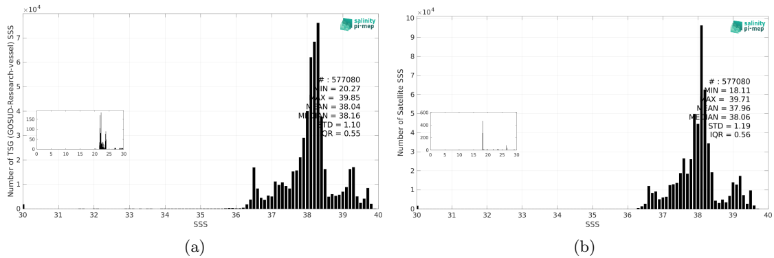
Figure 3: Histograms of SSS from TSG (GOSUD-Research-vessel) (a) and SMOS SSS L4 v1 - Monthly (CMEMS-CNR) (b) considering all match-up pairs per bins of 0.1 over the Mediterranean Sea Pi-MEP region and for the full satellite product period.
