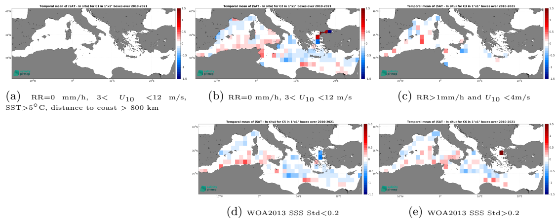
Figure 14: Temporal mean gridded over spatial boxes of size 1^\circ \times 1^\circ of \Delta SSS (SMOS SSS L4 v1 - Monthly (CMEMS-CNR) - TSG (GOSUD-Research-vessel)) for 5 different subdatasets corresponding to:RR=0 mm/h, 3 < U_{10} < 12 m/s, SST>5°C, distance to coast > 800 km (a), RR=0 mm/h, 3 < U_{10} < 12 m/s (b), RR>1mm/h and U_{10} < 4 m/s (c), WOA2013 SSS Std<0.2 (d), WOA2013 SSS Std>0.2 (e).
