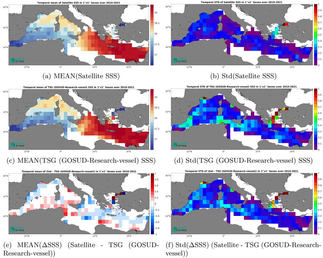
Figure 7: Temporal mean (left) and Std (right) of SSS from SMOS SSS L4 v1 - Monthly (CMEMS-CNR) (top), TSG (GOSUD-Research-vessel) (middle), and of \Delta\text{SSS} (Satellite - TSG (GOSUD-Research-vessel)). Only match-up pairs are used to generate these maps.
