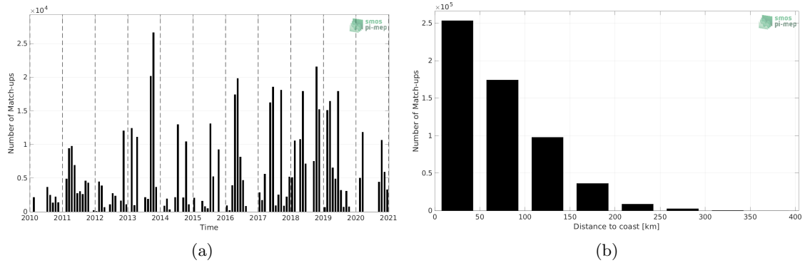
Figure 1: Number of match-ups between TSG (GOSUD-Research-vessel) and SMOS SSS L4 v1 - Monthly (CMEMS-CNR) SSS as a function of time (a) and as function of the distance to coast (b) over the Mediterranean Sea Pi-MEP region and for the full satellite product period.
