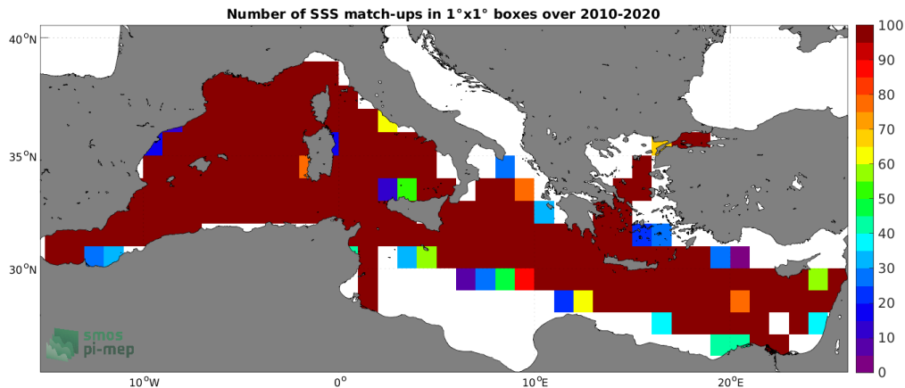
Figure 4: Number of SSS match-ups between TSG (GOSUD-Research-vessel) SSS and the SMOS SSS L4 v1 - Monthly (CMEMS-CNR) SSS product for the Mediterranean Sea Pi-MEP region over 1^\circ \times 1^\circ boxes and for the full satellite product period.
