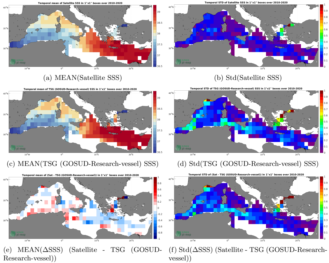
Figure 6: Temporal mean (left) and Std (right) of SSS from SMOS SSS L4 v1 - Monthly (CMEMS-CNR) (top), TSG (GOSUD-Research-vessel) (middle), and of \Delta SSS (Satellite - TSG (GOSUD-Research-vessel)). Only match-up pairs are used to generate these maps.
