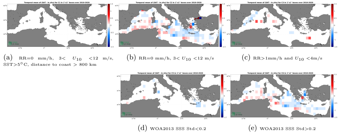
Figure 12: Temporal mean gridded over spatial boxes of size 1^{\circ}\times 1^{\circ} of \Delta SSS (SMOS SSS L4 v1 - Monthly (CMEMS-CNR) - TSG (GOSUD-Research-vessel)) for 5 different subdatasets corresponding to:RR=0 mm/h, 3 < U_{10} < 12 m/s, SST >5^{\circ}\text{C} , distance to coast > 800 km (a), RR=0 mm/h, 3 < U_{10} < 12 m/s (b), RR >1 mm/h and U_{10} < 4 m/s (c), WOA2013 SSS Std <0.2 (d), WOA2013 SSS Std >0.2 (e).
