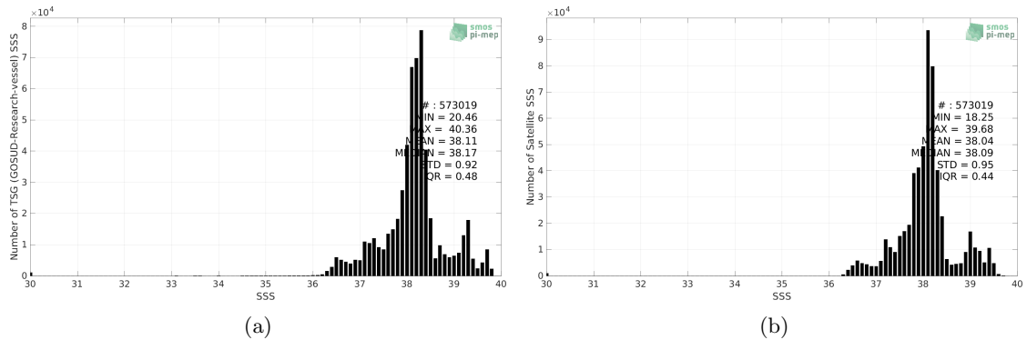
Figure 2: Histograms of SSS from TSG (GOSUD-Research-vessel) (a) and SMOS SSS L4 v1 - Monthly (CMEMS-CNR) (b) considering all match-up pairs per bins of 0.1 over the Mediterranean Sea Pi-MEP region and for the full satellite product period.
