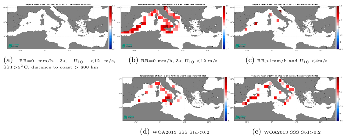
Figure 14: Temporal mean gridded over spatial boxes of size 1^\circ \times 1^\circ of \Delta SSS (SMOS SSS L4 v1 - Monthly (CMEMS-CNR) - Saildrone) for 5 different subdatasets corresponding to:RR=0 mm/h, 3 < U_{10} < 12 m/s, SST>5°C, distance to coast > 800 km (a), RR=0 mm/h, 3 < U_{10} < 12 m/s (b), RR>1mm/h and U_{10} < 4 m/s (c), WOA2013 SSS Std<0.2 (d), WOA2013 SSS Std>0.2 (e).
