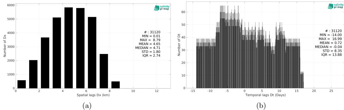
Figure 5: Histograms of the spatial (a) and temporal (b) lags between the location/time of the Saildrone measurement and the date of the corresponding SMOS SSS L4 v1 - Monthly (CMEMS-CNR) SSS pixel.
