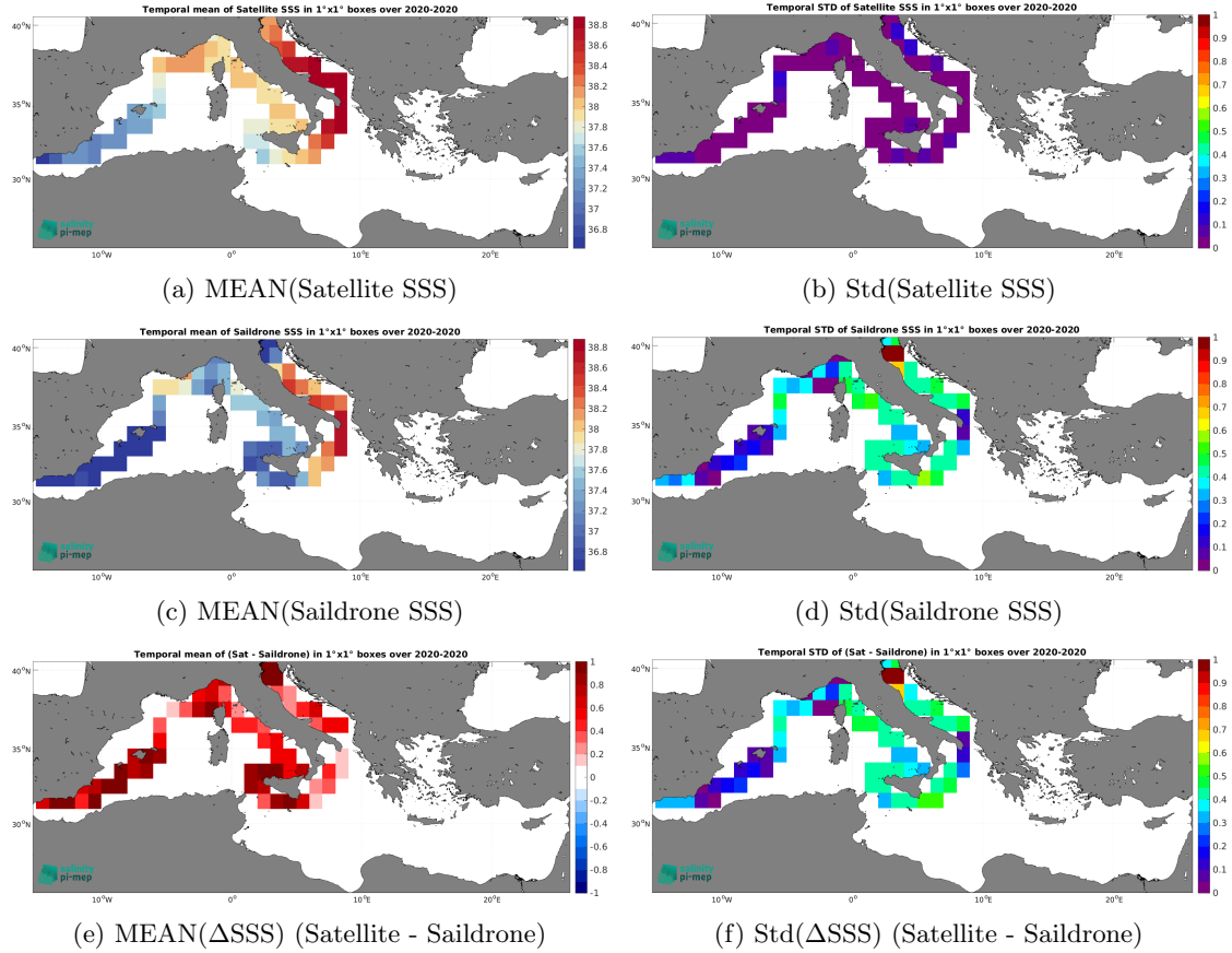
Figure 6: Temporal mean (left) and Std (right) of SSS from SMOS SSS L4 v1 - Monthly (CMEMS-CNR) (top), Saildrone (middle), and of \Delta\text{SSS} (Satellite - Saildrone). Only match-up pairs are used to generate these maps.
