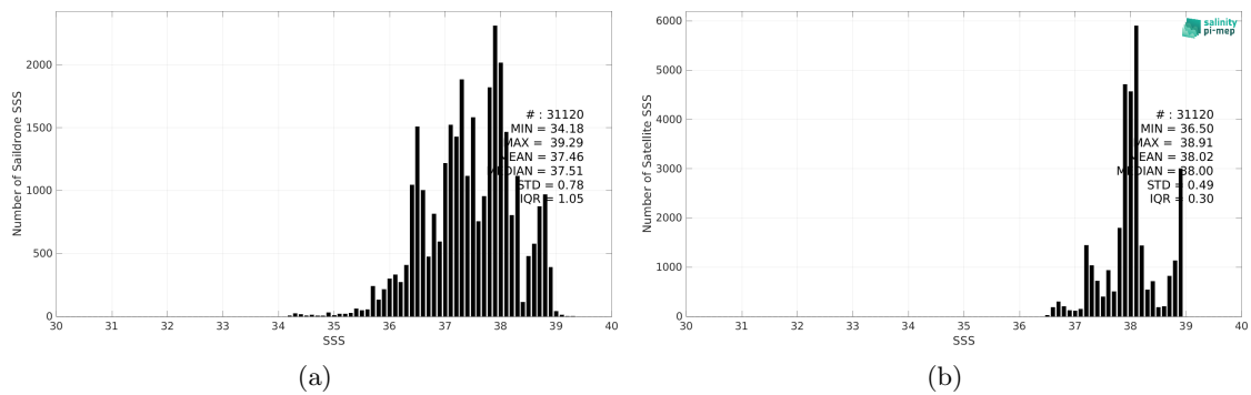
Figure 2: Histograms of SSS from Saildrone (a) and SMOS SSS L4 v1 - Monthly (CMEMS-CNR) (b) considering all match-up pairs per bins of 0.1 over the Mediterranean Sea Pi-MEP region and for the full satellite product period.
