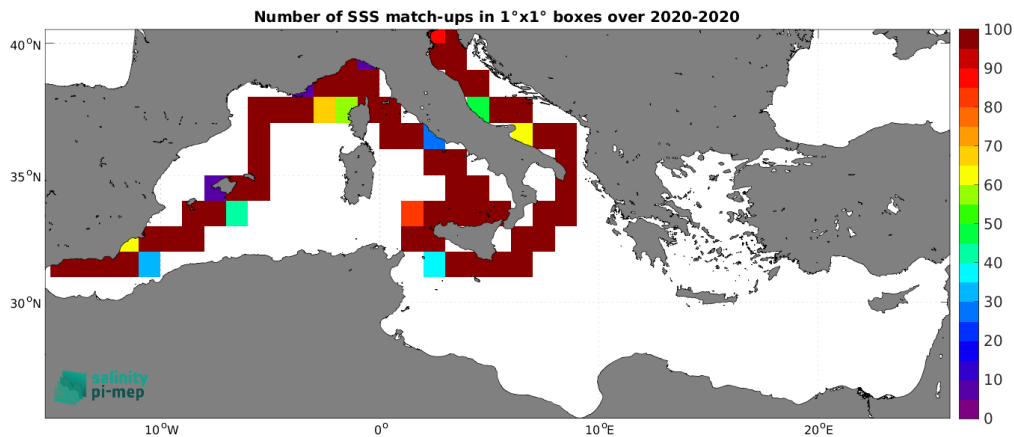
Figure 4: Number of SSS match-ups between Saildrone SSS and the SMOS SSS L4 v1 - Monthly (CMEMS-CNR) SSS product for the Mediterranean Sea Pi-MEP region over 1^\circ \times 1^\circ boxes and for the full satellite product period.
