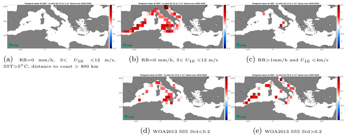
Figure 12: Temporal mean gridded over spatial boxes of size 1^\circ \times 1^\circ of \Delta SSS (SMOS SSS L4 v1 - Monthly (CMEMS-CNR) - Saildrone) for 5 different subdatasets corresponding to:RR=0 mm/h, 3 < U_{10} < 12 m/s, SST >5^\circ\text{C} , distance to coast > 800 km (a), RR=0 mm/h, 3 < U_{10} < 12 m/s (b), RR >1 mm/h and U_{10} < 4 m/s (c), WOA2013 SSS Std <0.2 (d), WOA2013 SSS Std >0.2 (e).
