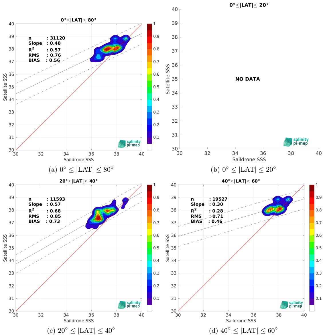
Figure 9: Contour maps of the concentration of SMOS SSS L4 v1 - Monthly (CMEMS-CNR) SSS (y-axis) versus Saildrone SSS (x-axis) at match-up pairs for different latitude bands. For each plot, the red line shows x=y . The black thin and dashed lines indicate a linear fit through the data cloud and the \pm 95\% confidence levels, respectively. The number match-up pairs n , the slope and R^2 coefficient of the linear fit, the root mean square (RMS) and the mean bias between satellite and in situ data are indicated for each latitude band in each plots.
