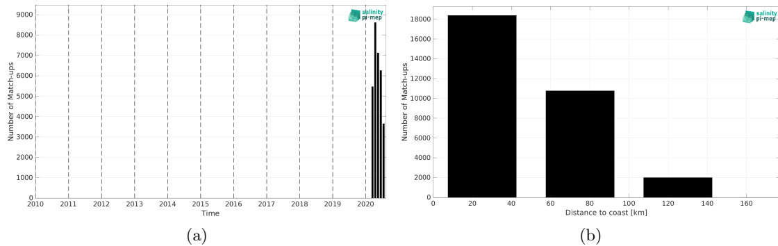
Figure 1: Number of match-ups between Saildrone and SMOS SSS L4 v1 - Monthly (CMEMS-CNR) SSS as a function of time (a) and as function of the distance to coast (b) over the Mediterranean Sea Pi-MEP region and for the full satellite product period.
