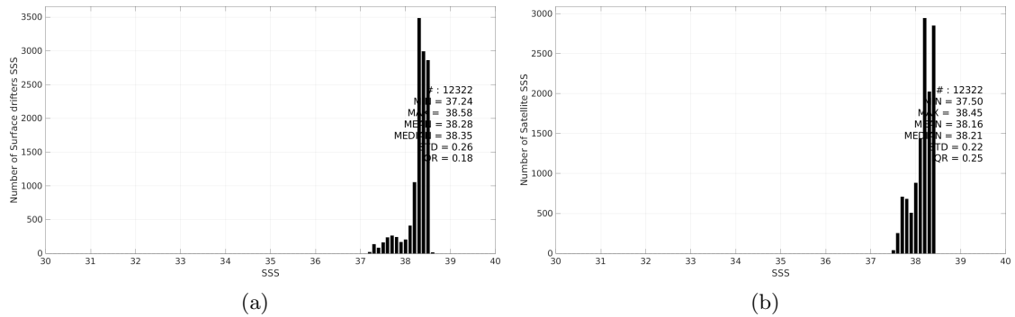
Figure 3: Histograms of SSS from Surface drifters (a) and SMOS SSS L4 v1 - Monthly (CMEMS-CNR) (b) considering all match-up pairs per bins of 0.1 over the Mediterranean Sea Pi-MEP region and for the full satellite product period.
