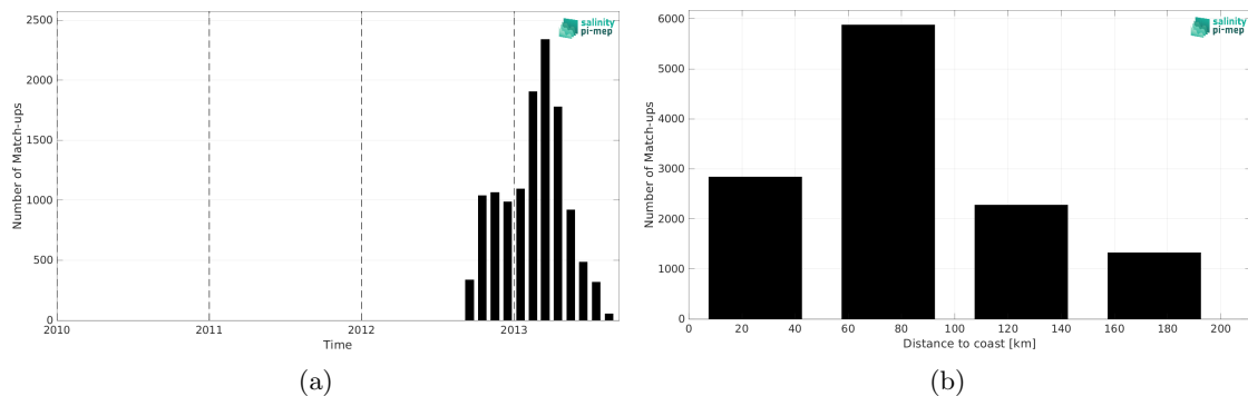
Figure 2: Number of match-ups between Surface drifters and SMOS SSS L4 v1 - Monthly (CMEMS-CNR) SSS as a function of time (a) and as function of the distance to coast (b) over the Mediterranean Sea Pi-MEP region and for the full satellite product period.
