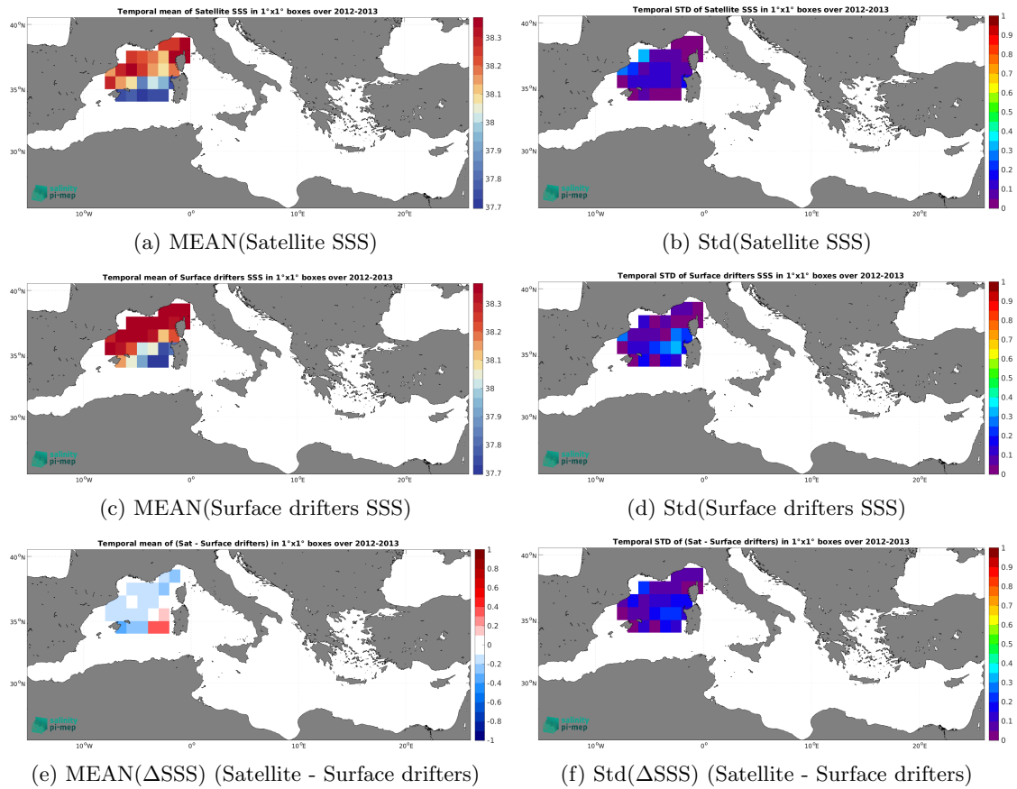
Figure 6: Temporal mean (left) and Std (right) of SSS from SMOS SSS L4 v1 - Monthly (CMEMS-CNR) (top), Surface drifters (middle), and of \Delta SSS (Satellite - Surface drifters). Only match-up pairs are used to generate these maps.
