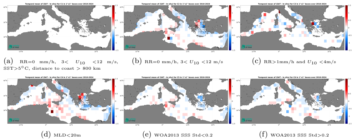
Figure 14: Temporal mean gridded over spatial boxes of size 1^\circ \times 1^\circ of \Delta SSS (SMOS SSS L4 v1 - Monthly (CMEMS-CNR) - Argo) for 6 different subdatasets corresponding to:RR=0 mm/h, 3 < U_{10} < 12 m/s, SST >5^\circ C, distance to coast > 800 km (a), RR=0 mm/h, 3 < U_{10} < 12 m/s (b), RR >1 mm/h and U_{10} < 4 m/s (c),MLD <20 m (d),WOA2013 SSS Std <0.2 (e),WOA2013 SSS Std >0.2 (f).
