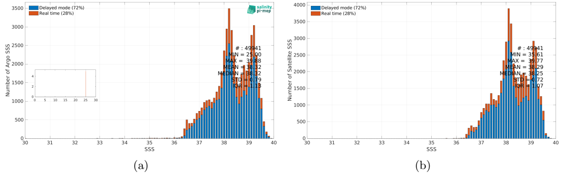
Figure 3: Histograms of SSS from Argo (a) and SMOS SSS L4 v1 - Monthly (CMEMS-CNR) (b) considering all match-up pairs per bins of 0.1 over the Mediterranean Sea Pi-MEP region and for the full satellite product period.
