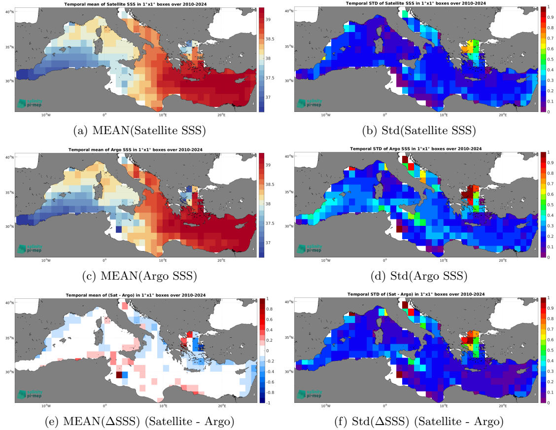
Figure 7: Temporal mean (left) and Std (right) of SSS from SMOS SSS L4 v1 - Monthly (CMEMS-CNR) (top), Argo (middle), and of \Delta\text{SSS} (Satellite - Argo). Only match-up pairs are used to generate these maps.
