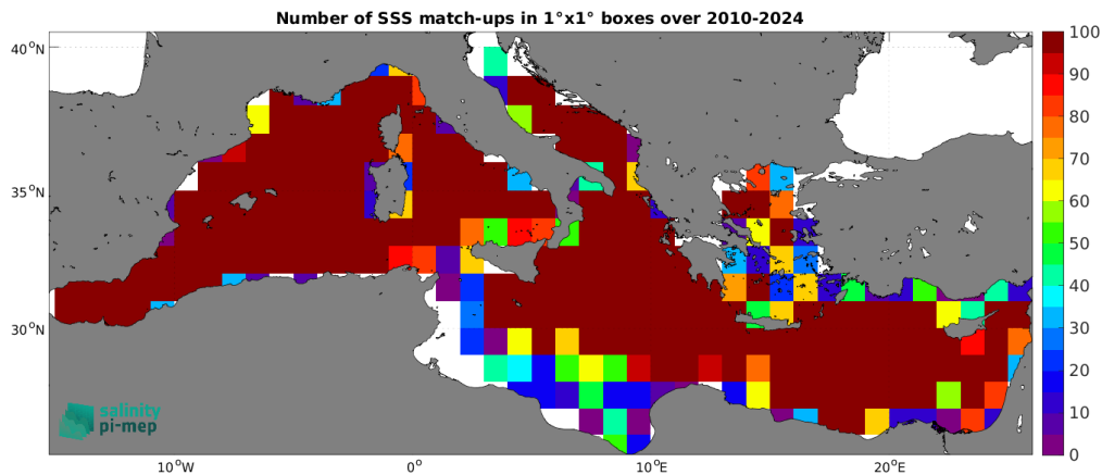
Figure 5: Number of SSS match-ups between Argo SSS and the SMOS SSS L4 v1 - Monthly (CMEMS-CNR) SSS product for the Mediterranean Sea Pi-MEP region over 1^\circ \times 1^\circ boxes and for the full satellite product period.
