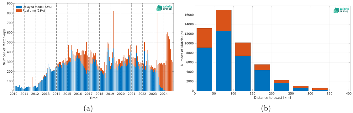
Figure 2: Number of match-ups between Argo and SMOS SSS L4 v1 - Monthly (CMEMS-CNR) SSS as a function of time (a) and as function of the distance to coast (b) over the Mediterranean Sea Pi-MEP region and for the full satellite product period.
