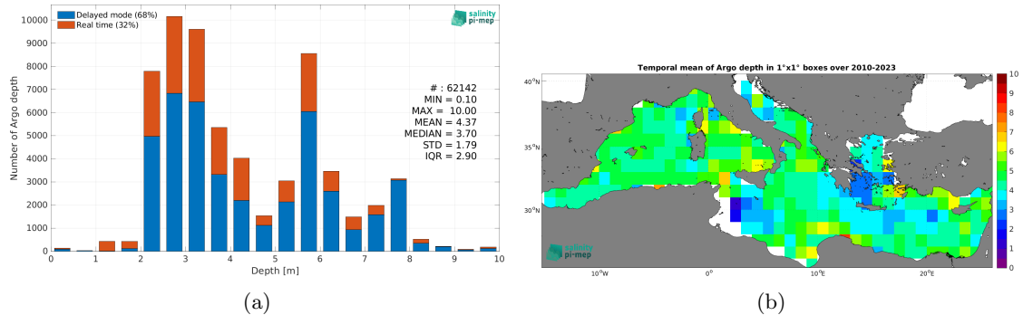
Figure 3: Histograms of the depth of the upper level SSS measurements from Argo in the Match-up DataBase for the Mediterranean Sea Pi-MEP region (a) and temporal mean spatial distribution of pressure of the in situ SSS data over 1^\circ \times 1^\circ boxes and for the full satellite product period (b).
