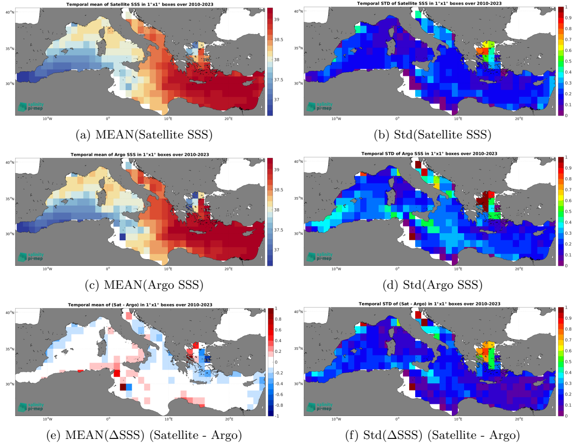
Figure 6: Temporal mean (left) and Std (right) of SSS from SMOS SSS L4 v1 - Monthly (CMEMS-CNR) (top), Argo (middle), and of \Delta\text{SSS} (Satellite - Argo). Only match-up pairs are used to generate these maps.
