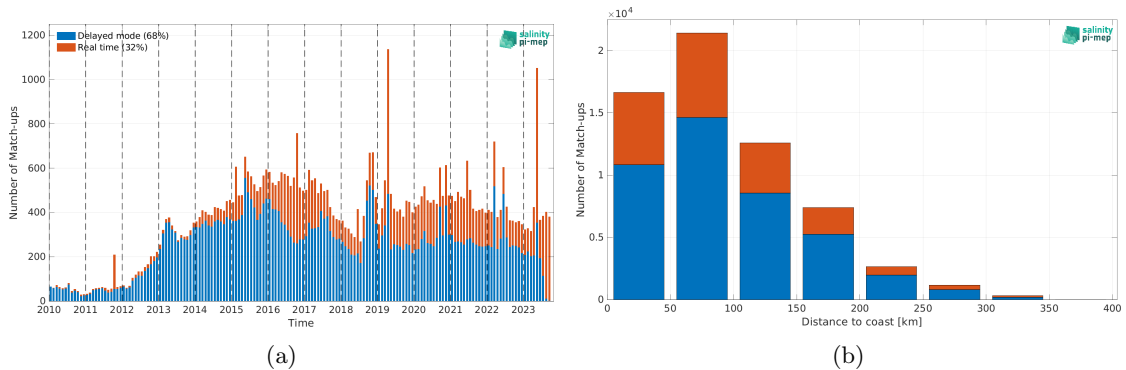
Figure 1: Number of match-ups between Argo and SMOS SSS L4 v1 - Monthly (CMEMS-CNR) SSS as a function of time (a) and as function of the distance to coast (b) over the Mediterranean Sea Pi-MEP region and for the full satellite product period.
