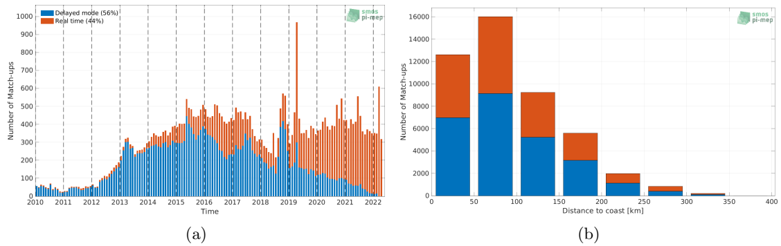
Figure 1: Number of match-ups between Argo and SMOS SSS L4 v1 - Monthly (CMEMS-CNR) SSS as a function of time (a) and as function of the distance to coast (b) over the Mediterranean Sea Pi-MEP region and for the full satellite product period.
