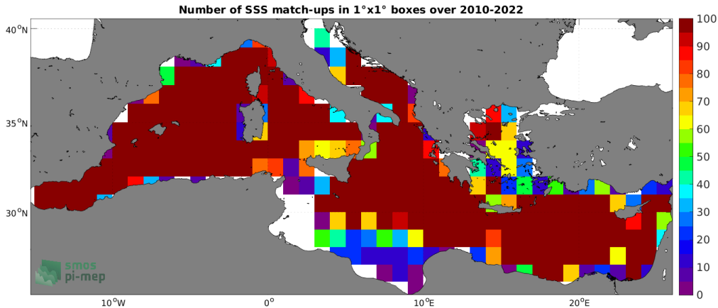
Figure 4: Number of SSS match-ups between Argo SSS and the SMOS SSS L4 v1 - Monthly (CMEMS-CNR) SSS product for the Mediterranean Sea Pi-MEP region over 1^\circ \times 1^\circ boxes and for the full satellite product period.
