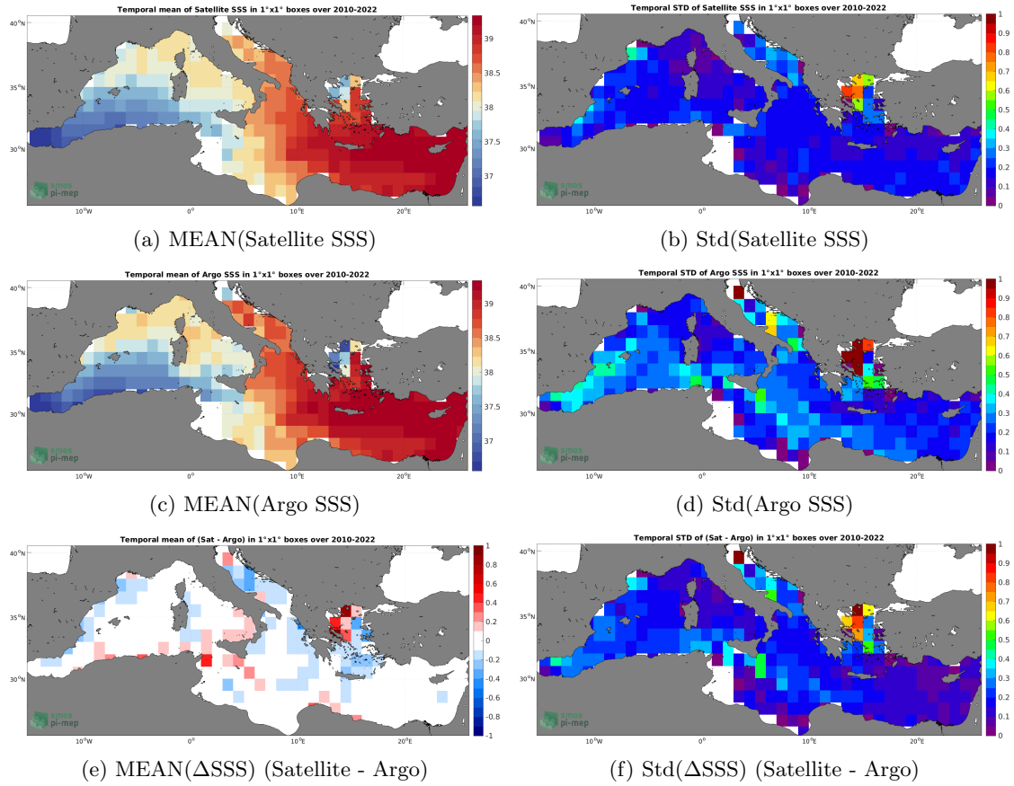
Figure 6: Temporal mean (left) and Std (right) of SSS from SMOS SSS L4 v1 - Monthly (CMEMS-CNR) (top), Argo (middle), and of \Delta SSS (Satellite - Argo). Only match-up pairs are used to generate these maps.
