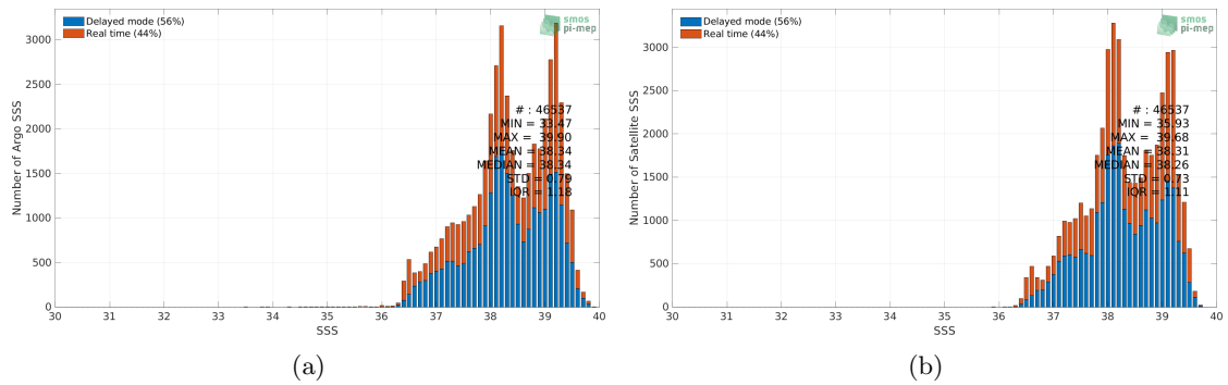
Figure 2: Histograms of SSS from Argo (a) and SMOS SSS L4 v1 - Monthly (CMEMS-CNR) (b) considering all match-up pairs per bins of 0.1 over the Mediterranean Sea Pi-MEP region and for the full satellite product period.
