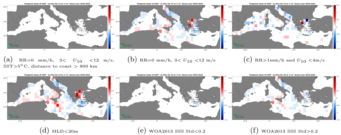
Figure 12: Temporal mean gridded over spatial boxes of size 1^\circ \times 1^\circ of \Delta SSS (SMOS SSS L4 v1 - Monthly (CMEMS-CNR) - Argo) for 6 different subdatasets corresponding to:RR=0 mm/h, 3 < U_{10} < 12 m/s, SST >5^\circ C, distance to coast > 800 km (a), RR=0 mm/h, 3 < U_{10} < 12 m/s (b), RR >1 mm/h and U_{10} < 4 m/s (c),MLD <20 m (d),WOA2013 SSS Std <0.2 (e),WOA2013 SSS Std >0.2 (f).
