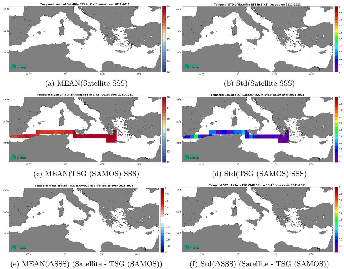
Figure 6: Temporal mean (left) and Std (right) of SSS from SMOS SSS L4 v1 - Daily (CMEMS-CNR) (top), TSG (SAMOS) (middle), and of \Delta SSS (Satellite - TSG (SAMOS)). Only match-up pairs are used to generate these maps.
