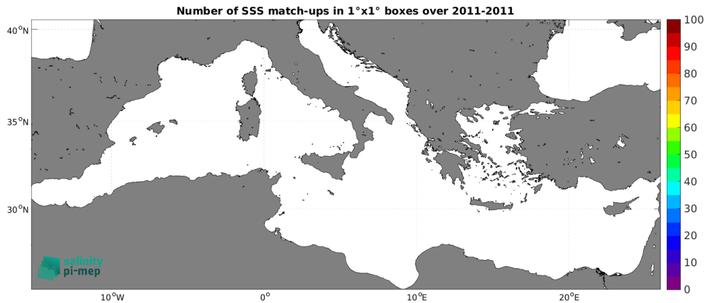
Figure 4: Number of SSS match-ups between TSG (SAMOS) SSS and the SMOS SSS L4 v1 - Daily (CMEMS-CNR) SSS product for the Mediterranean Sea Pi-MEP region over 1^\circ \times 1^\circ boxes and for the full satellite product period.
