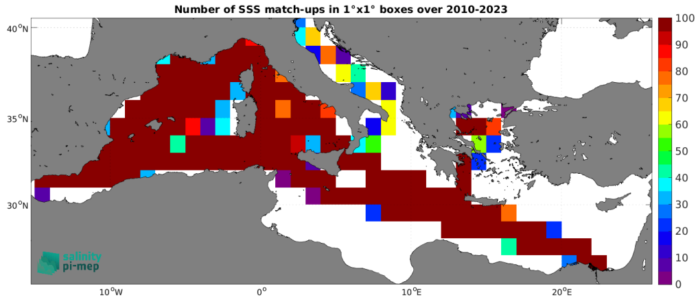
Figure 5: Number of SSS match-ups between TSG (LEGOS-DM) SSS and the SMOS SSS L4 v1 - Daily (CMEMS-CNR) SSS product for the Mediterranean Sea Pi-MEP region over 1^\circ \times 1^\circ boxes and for the full satellite product period.
