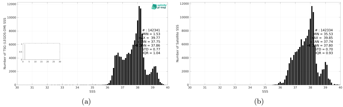
Figure 3: Histograms of SSS from TSG (LEGOS-DM) (a) and SMOS SSS L4 v1 - Daily (CMEMS-CNR) (b) considering all match-up pairs per bins of 0.1 over the Mediterranean Sea Pi-MEP region and for the full satellite product period.
