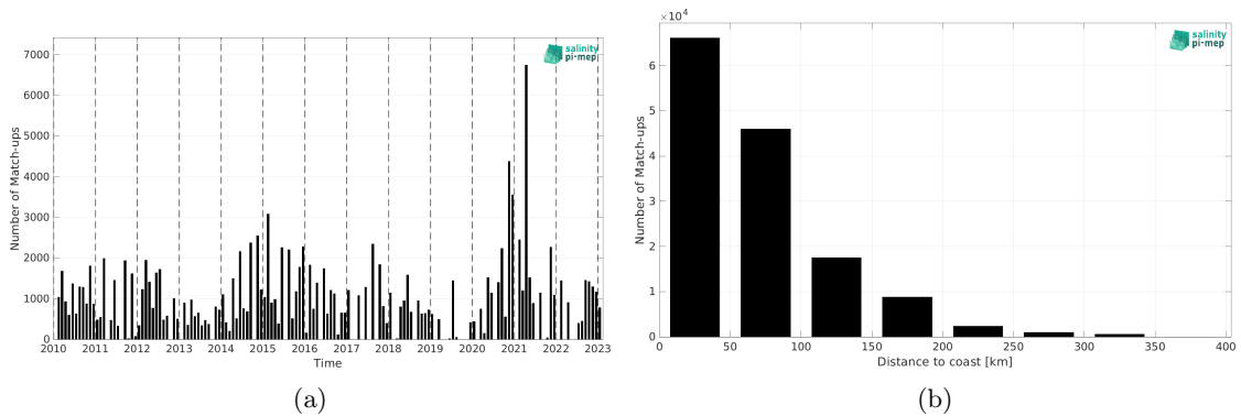
Figure 2: Number of match-ups between TSG (LEGOS-DM) and SMOS SSS L4 v1 - Daily (CMEMS-CNR) SSS as a function of time (a) and as function of the distance to coast (b) over the Mediterranean Sea Pi-MEP region and for the full satellite product period.
