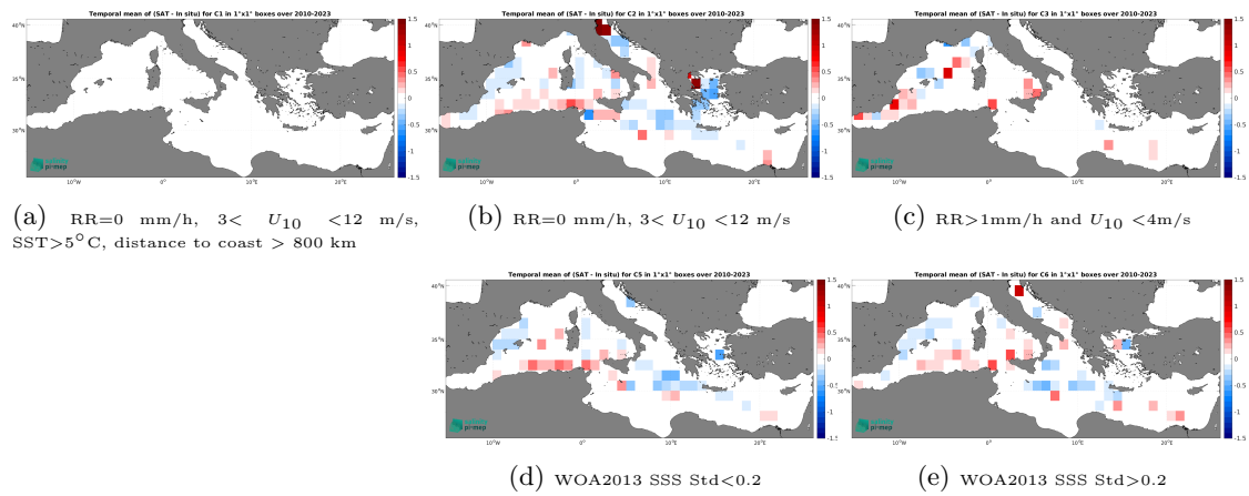
Figure 14: Temporal mean gridded over spatial boxes of size 1^\circ \times 1^\circ of \Delta SSS (SMOS SSS L4 v1 - Daily (CMEMS-CNR) - TSG (LEGOS-DM)) for 5 different subdatasets corresponding to:RR=0 mm/h, 3 < U_{10} < 12 m/s, SST >5^\circ\text{C} , distance to coast > 800 km (a), RR=0 mm/h, 3 < U_{10} < 12 m/s (b), RR >1 mm/h and U_{10} < 4 m/s (c), WOA2013 SSS Std <0.2 (d), WOA2013 SSS Std >0.2 (e).
