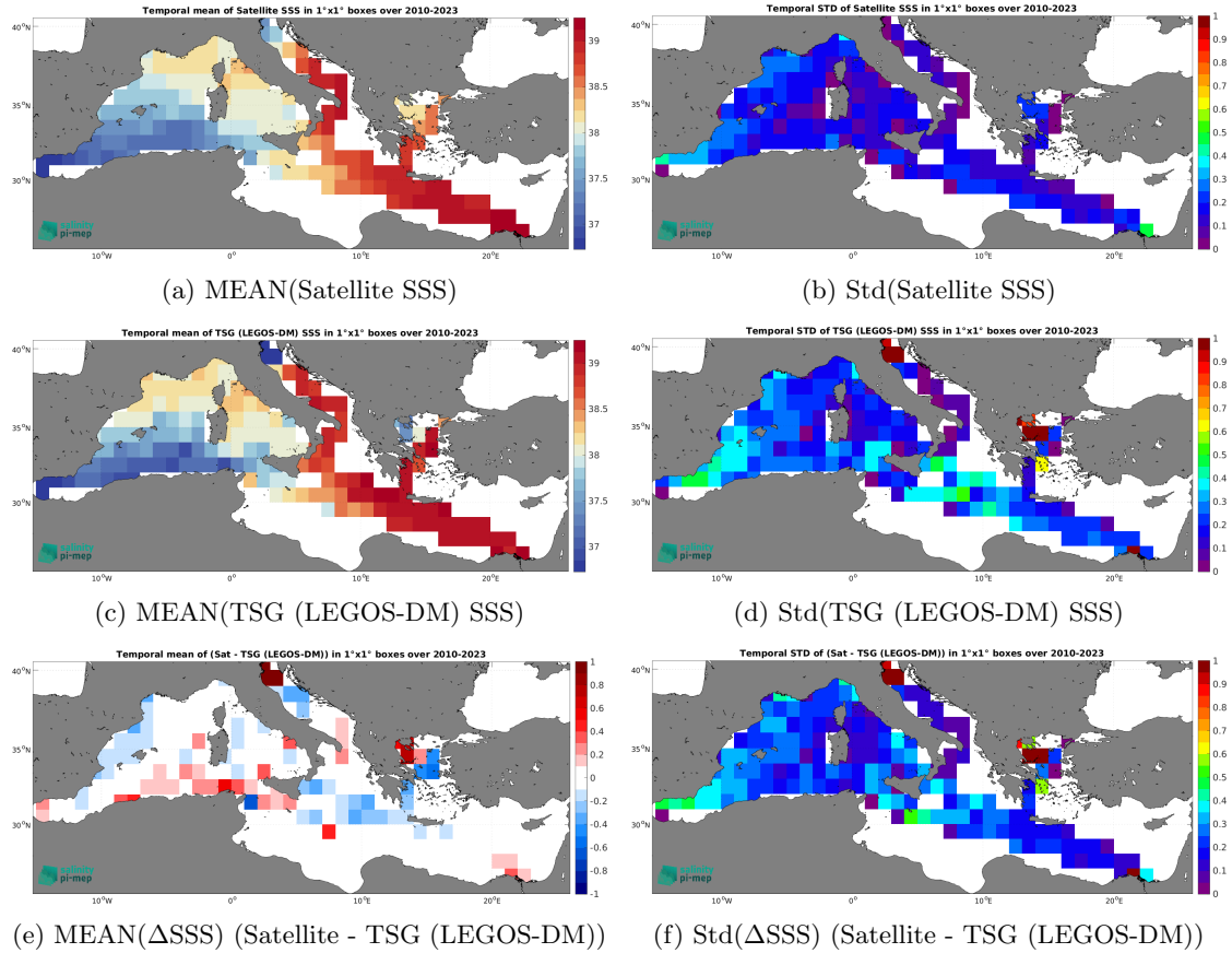
Figure 7: Temporal mean (left) and Std (right) of SSS from SMOS SSS L4 v1 - Daily (CMEMS-CNR) (top), TSG (LEGOS-DM) (middle), and of \Delta\text{SSS} (Satellite - TSG (LEGOS-DM)). Only match-up pairs are used to generate these maps.
