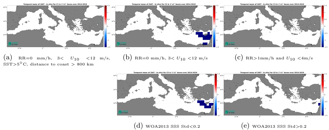
Figure 14: Temporal mean gridded over spatial boxes of size 1^\circ \times 1^\circ of \Delta SSS (SMOS SSS L4 v1 - Daily (CMEMS-CNR) - TSG (GOSUD-Sailing-ship)) for 5 different subdatasets corresponding to:RR=0 mm/h, 3 < U_{10} < 12 m/s, SST>5°C, distance to coast > 800 km (a), RR=0 mm/h, 3 < U_{10} < 12 m/s (b), RR>1mm/h and U_{10} < 4 m/s (c), WOA2013 SSS Std<0.2 (d), WOA2013 SSS Std>0.2 (e).
