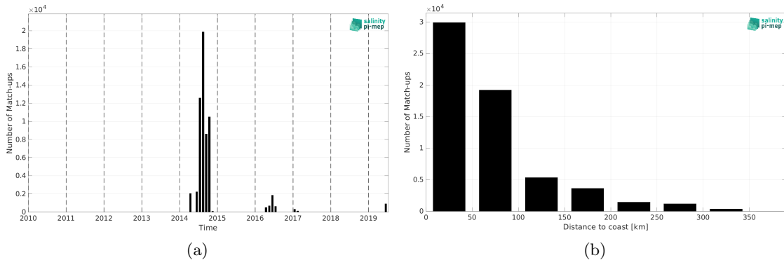
Figure 2: Number of match-ups between TSG (GOSUD-Sailing-ship) and SMOS SSS L4 v1 - Daily (CMEMS-CNR) SSS as a function of time (a) and as function of the distance to coast (b) over the Mediterranean Sea Pi-MEP region and for the full satellite product period.
