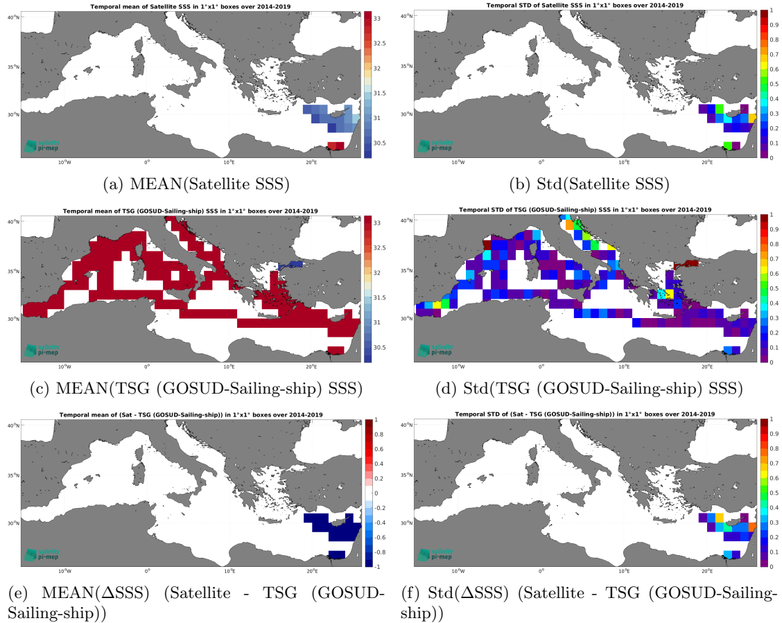
Figure 7: Temporal mean (left) and Std (right) of SSS from SMOS SSS L4 v1 - Daily (CMEMS-CNR) (top), TSG (GOSUD-Sailing-ship) (middle), and of \Delta\text{SSS} (Satellite - TSG (GOSUD-Sailing-ship)). Only match-up pairs are used to generate these maps.
