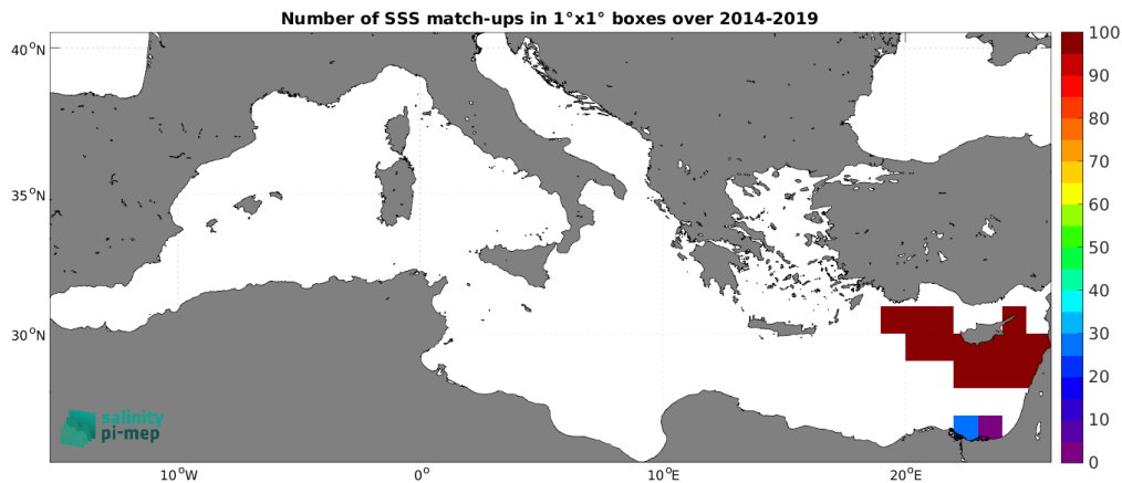
Figure 5: Number of SSS match-ups between TSG (GOSUD-Sailing-ship) SSS and the SMOS SSS L4 v1 - Daily (CMEMS-CNR) SSS product for the Mediterranean Sea Pi-MEP region over 1^\circ \times 1^\circ boxes and for the full satellite product period.
