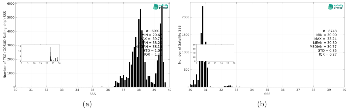
Figure 3: Histograms of SSS from TSG (GOSUD-Sailing-ship) (a) and SMOS SSS L4 v1 - Daily (CMEMS-CNR) (b) considering all match-up pairs per bins of 0.1 over the Mediterranean Sea Pi-MEP region and for the full satellite product period.
