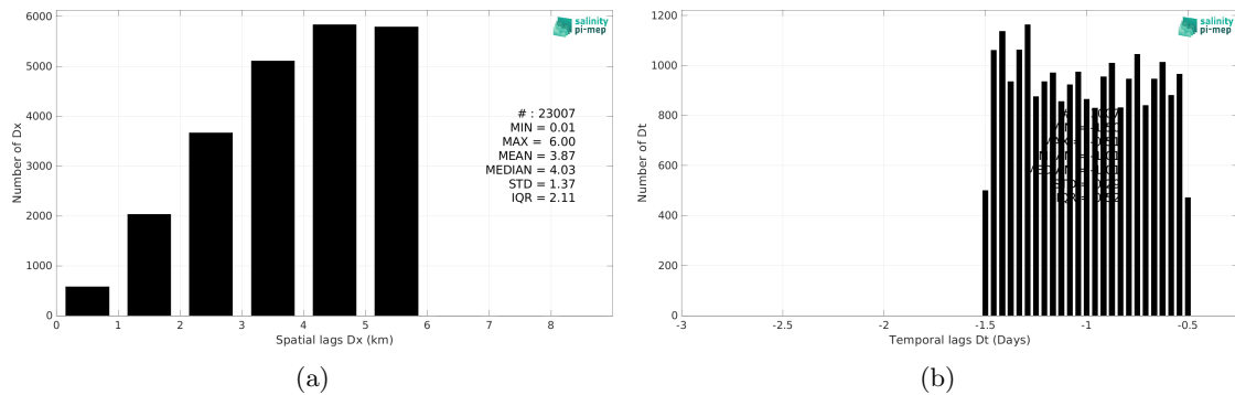
Figure 6: Histograms of the spatial (a) and temporal (b) lags between the location/time of the Saildrone measurement and the date of the corresponding SMOS SSS L4 v1 - Daily (CMEMS-CNR) SSS pixel.
