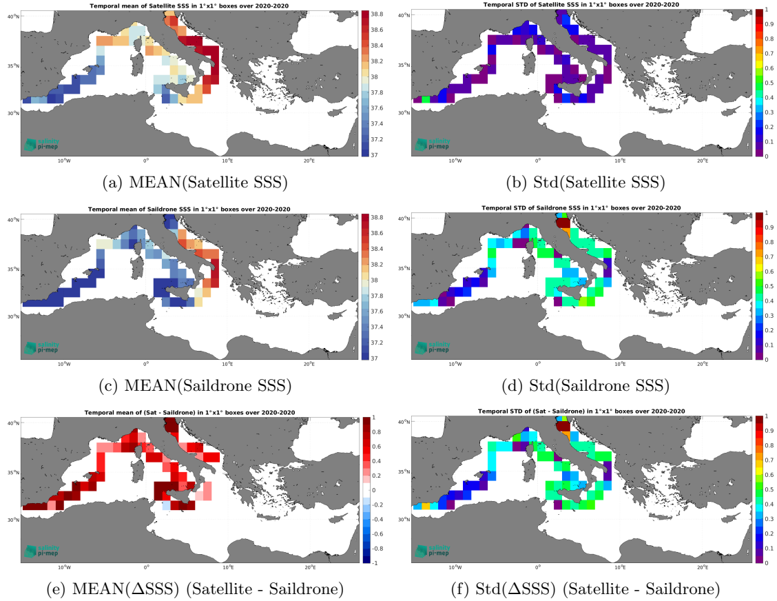
Figure 7: Temporal mean (left) and Std (right) of SSS from SMOS SSS L4 v1 - Daily (CMEMS-CNR) (top), Saildrone (middle), and of \Delta SSS (Satellite - Saildrone). Only match-up pairs are used to generate these maps.
