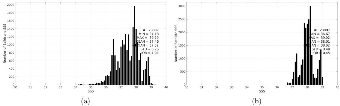
Figure 3: Histograms of SSS from Saildrone (a) and SMOS SSS L4 v1 - Daily (CMEMS-CNR) (b) considering all match-up pairs per bins of 0.1 over the Mediterranean Sea Pi-MEP region and for the full satellite product period.
