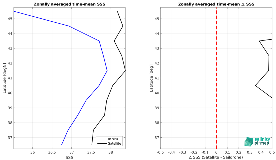
Figure 9: Left panel: Zonal mean SSS from SMOS SSS L4 v1 - Daily (CMEMS-CNR) satellite product (black) and from Sairdron (blue). Right panel: Zonal mean of \Delta SSS (Satellite - Sairdron) for all the collected Pi-MEP match-up pairs estimated over the full satellite product period.
