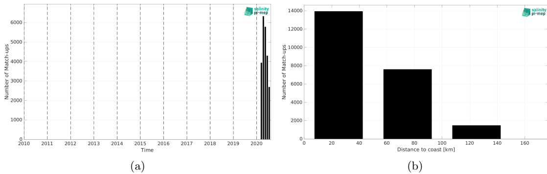
Figure 2: Number of match-ups between Saildrone and SMOS SSS L4 v1 - Daily (CMEMS-CNR) SSS as a function of time (a) and as function of the distance to coast (b) over the Mediterranean Sea Pi-MEP region and for the full satellite product period.
