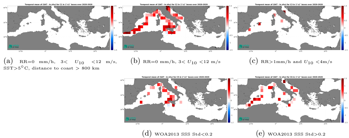
Figure 14: Temporal mean gridded over spatial boxes of size 1^\circ \times 1^\circ of \Delta\text{SSS} (SMOS SSS L4 v1 - Daily (CMEMS-CNR) - Saildrone) for 5 different subdatasets corresponding to:RR=0 mm/h, 3 < U_{10} < 12 m/s, SST>5°C, distance to coast > 800 km (a), RR=0 mm/h, 3 < U_{10} < 12 m/s (b), RR>1mm/h and U_{10} < 4 m/s (c), WOA2013 SSS Std<0.2 (d), WOA2013 SSS Std>0.2 (e).
