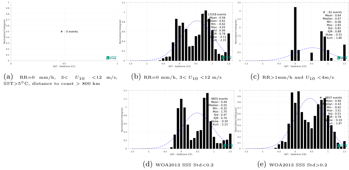
Figure 15: Normalized histogram of \Delta SSS (SMOS SSS L4 v1 - Daily (CMEMS-CNR) - Saildrone) for 5 different subdatasets corresponding to: RR=0 mm/h, 3 < U_{10} < 12 m/s, SST > 5°C, distance to coast > 800 km (a), RR=0 mm/h, 3 < U_{10} < 12 m/s (b), RR > 1mm/h and U_{10} < 4 m/s (c), WOA2013 SSS Std < 0.2 (d), WOA2013 SSS Std > 0.2 (e).
