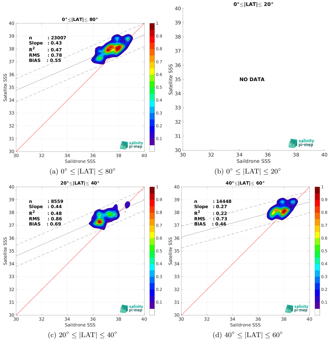
Figure 10: Contour maps of the concentration of SMOS SSS L4 v1 - Daily (CMEMS-CNR) SSS (y-axis) versus Saildrone SSS (x-axis) at match-up pairs for different latitude bands. For each plot, the red line shows x=y . The black thin and dashed lines indicate a linear fit through the data cloud and the \pm 95\% confidence levels, respectively. The number match-up pairs n , the slope and R^2 coefficient of the linear fit, the root mean square (RMS) and the mean bias between satellite and in situ data are indicated for each latitude band in each plots.
