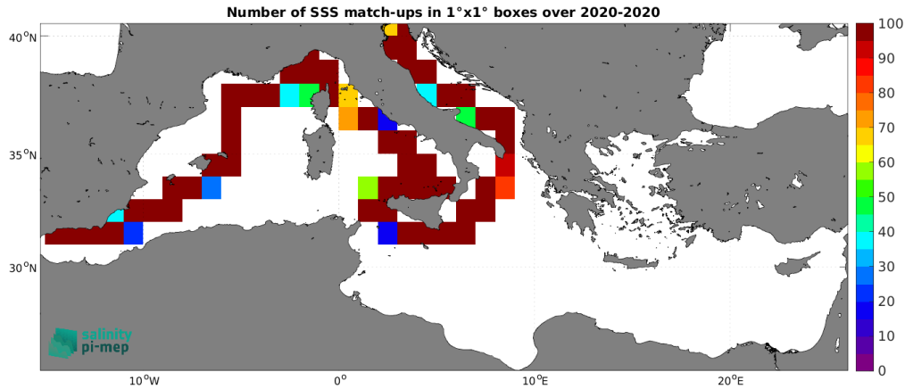
Figure 5: Number of SSS match-ups between Saildrone SSS and the SMOS SSS L4 v1 - Daily (CMEMS-CNR) SSS product for the Mediterranean Sea Pi-MEP region over 1^\circ \times 1^\circ boxes and for the full satellite product period.
