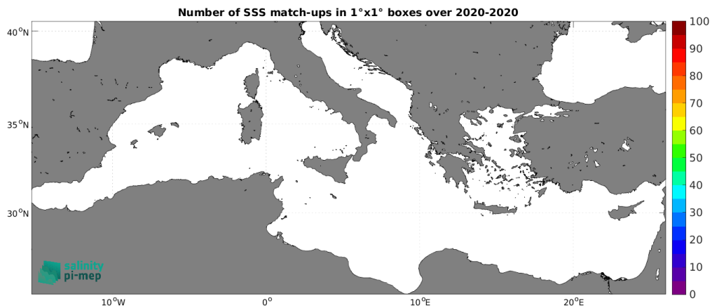
Figure 4: Number of SSS match-ups between Saildrone SSS and the SMOS SSS L4 v1 - Daily (CMEMS-CNR) SSS product for the Mediterranean Sea Pi-MEP region over 1^\circ \times 1^\circ boxes and for the full satellite product period.
