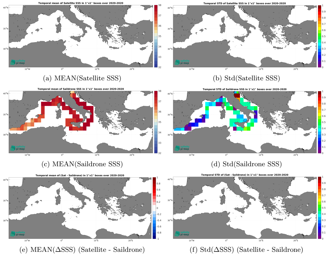
Figure 6: Temporal mean (left) and Std (right) of SSS from SMOS SSS L4 v1 - Daily (CMEMS-CNR) (top), Saildrone (middle), and of \Delta SSS (Satellite - Saildrone). Only match-up pairs are used to generate these maps.
