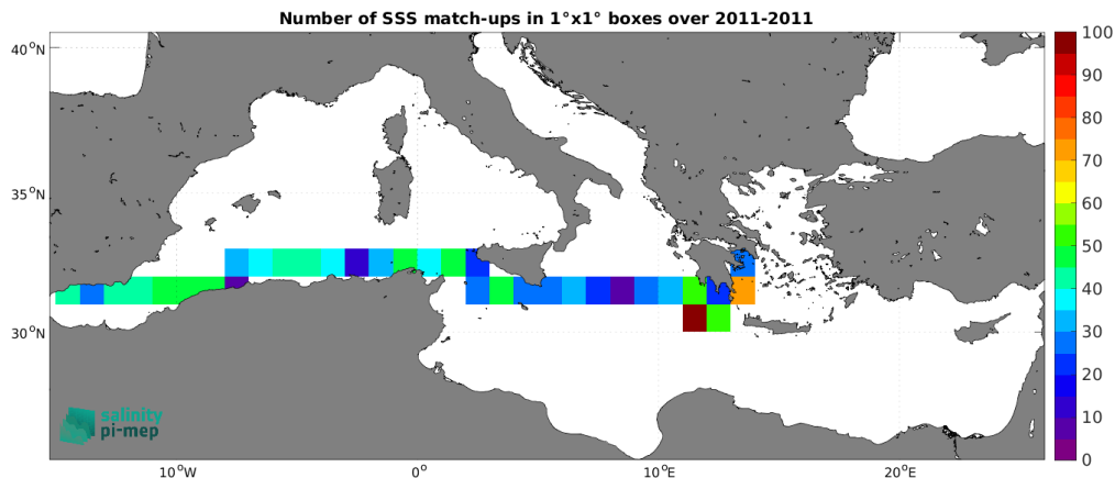
Figure 5: Number of SSS match-ups between TSG (SAMOS) SSS and the SMOS SSS L4 OI v346 - Weekly (CMEMS-CATDS-LOPS) SSS product for the Mediterranean Sea Pi-MEP region over 1^\circ \times 1^\circ boxes and for the full satellite product period.
