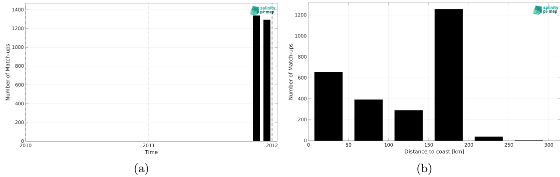
Figure 2: Number of match-ups between TSG (SAMOS) and SMOS SSS L4 OI v346 - Weekly (CMEMS-CATDS-LOPS) SSS as a function of time (a) and as function of the distance to coast (b) over the Mediterranean Sea Pi-MEP region and for the full satellite product period.
