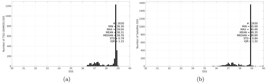
Figure 3: Histograms of SSS from TSG (SAMOS) (a) and SMOS SSS L4 OI v346 - Weekly (CMEMS-CATDS-LOPS) (b) considering all match-up pairs per bins of 0.1 over the Mediterranean Sea Pi-MEP region and for the full satellite product period.
