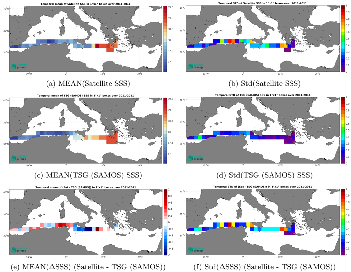
Figure 7: Temporal mean (left) and Std (right) of SSS from SMOS SSS L4 OI v346 - Weekly (CMEMS-CATDS-LOPS) (top), TSG (SAMOS) (middle), and of \Delta SSS (Satellite - TSG (SAMOS)). Only match-up pairs are used to generate these maps.
