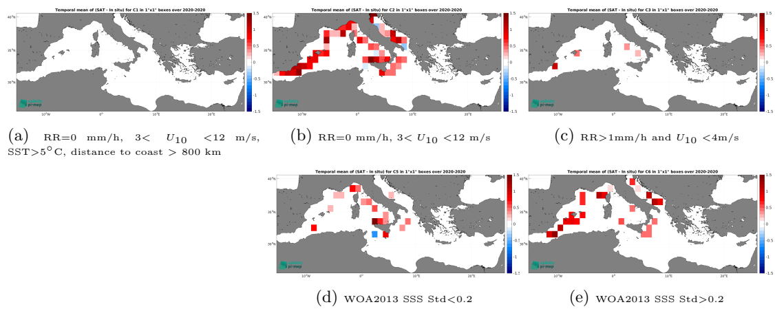
Figure 14: Temporal mean gridded over spatial boxes of size 1^\circ \times 1^\circ of \Delta\text{SSS} (SMOS SSS L4 OI v346 - Weekly (CMEMS-CATDS-LOPS) - Saildrone) for 5 different subdatasets corresponding to:RR=0 mm/h, 3 < U_{10} < 12 m/s, SST>5°C, distance to coast > 800 km (a), RR=0 mm/h, 3 < U_{10} < 12 m/s (b), RR>1mm/h and U_{10} < 4 m/s (c), WOA2013 SSS Std<0.2 (d), WOA2013 SSS Std>0.2 (e).
