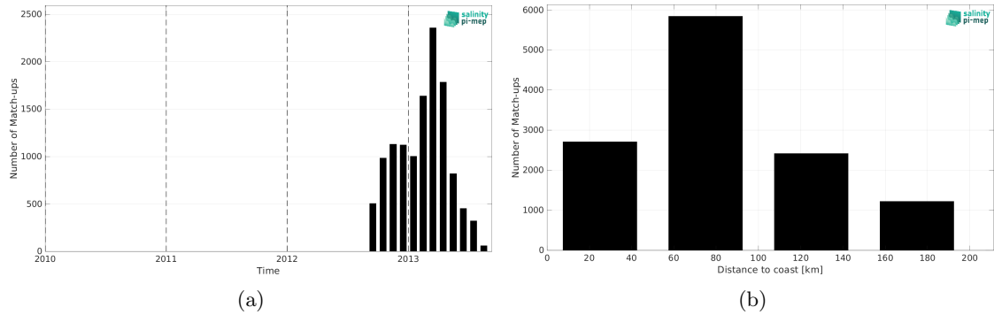
Figure 2: Number of match-ups between Surface drifters and SMOS SSS L4 OI v346 - Weekly (CMEMS-CATDS-LOPS) SSS as a function of time (a) and as function of the distance to coast (b) over the Mediterranean Sea Pi-MEP region and for the full satellite product period.
