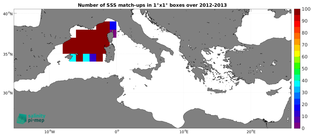
Figure 4: Number of SSS match-ups between Surface drifters SSS and the SMOS SSS L4 OI v346 - Weekly (CMEMS-CATDS-LOPS) SSS product for the Mediterranean Sea Pi-MEP region over 1^\circ \times 1^\circ boxes and for the full satellite product period.
