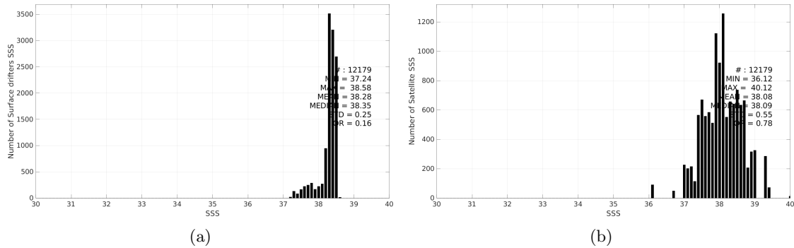
Figure 3: Histograms of SSS from Surface drifters (a) and SMOS SSS L4 OI v346 - Weekly (CMEMS-CATDS-LOPS) (b) considering all match-up pairs per bins of 0.1 over the Mediterranean Sea Pi-MEP region and for the full satellite product period.
