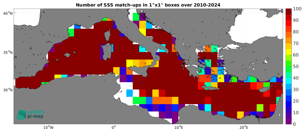
Figure 5: Number of SSS match-ups between Argo SSS and the SMOS SSS L4 OI v346 - Weekly (CMEMS-CATDS-LOPS) SSS product for the Mediterranean Sea Pi-MEP region over 1^\circ \times 1^\circ boxes and for the full satellite product period.
