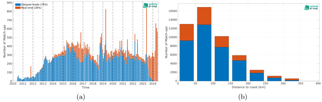
Figure 2: Number of match-ups between Argo and SMOS SSS L4 OI v346 - Weekly (CMEMS-CATDS-LOPS) SSS as a function of time (a) and as function of the distance to coast (b) over the Mediterranean Sea Pi-MEP region and for the full satellite product period.
