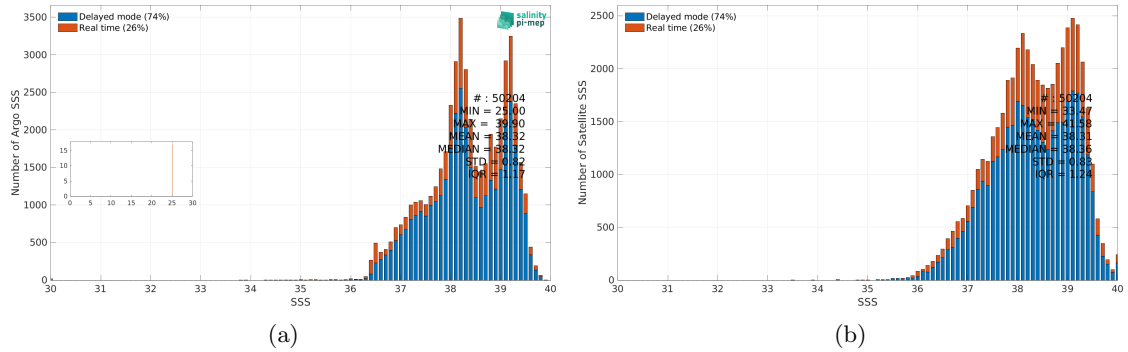
Figure 3: Histograms of SSS from Argo (a) and SMOS SSS L4 OI v346 - Weekly (CMEMS-CATDS-LOPS) (b) considering all match-up pairs per bins of 0.1 over the Mediterranean Sea Pi-MEP region and for the full satellite product period.
