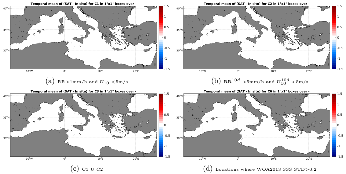
Figure 12: Temporal mean gridded over spatial boxes of size 1^\circ \times 1^\circ of \Delta SSS (SMOS-L4-CATDS-CECOS-IFREMER-V2-WEEKLY-0.5DEG - TSG-SAMOS) for 4 different subdatasets corresponding to: RR > 1\text{mm/h} and U_{10} < 5\text{m/s} (a), RR^{10d} > 5\text{mm/h} and U_{10}^{10d} < 5\text{m/s} (b), C1 U C2 (c), Locations where WOA2013 SSS STD > 0.2 (d).
