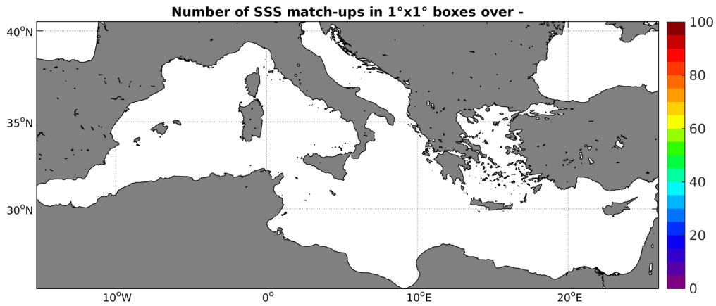
Figure 4: Number of SSS match-ups between TSG-SAMOS SSS and the SMOS-L4-CATDS-CECOS-IFREMER-V2-WEEKLY-0.5DEG SSS product for the Mediterranean Sea Pi-MEP region over 1^\circ \times 1^\circ boxes and for the full satellite product period.
