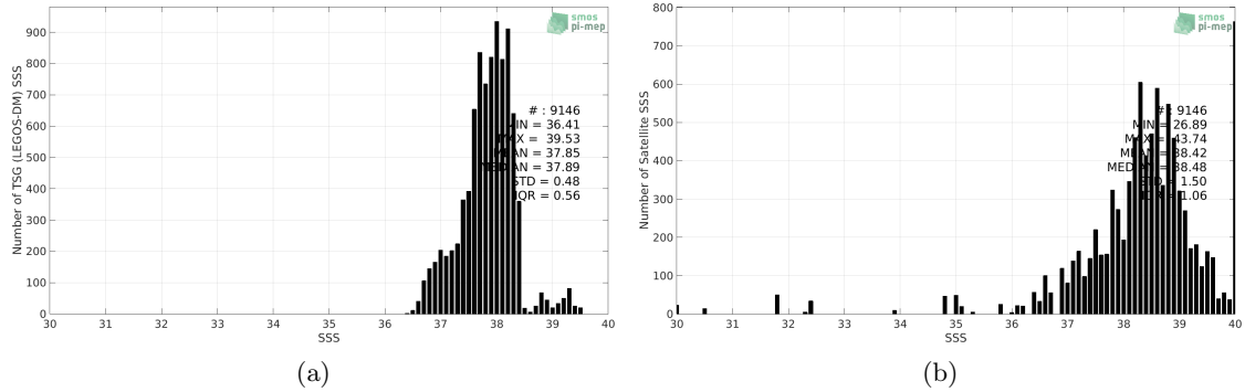
Figure 2: Histograms of SSS from TSG (LEGOS-DM) (a) and SMOS L4 v2 Weekly (CATDS-CECOS-IFREMER) (b) considering all match-up pairs per bins of 0.1 over the Mediterranean Sea Pi-MEP region and for the full satellite product period.
