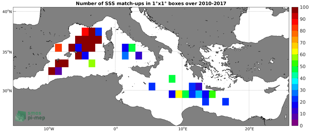
Figure 4: Number of SSS match-ups between TSG (LEGOS-DM) SSS and the SMOS L4 v2 Weekly (CATDS-CECOS-IFREMER) SSS product for the Mediterranean Sea Pi-MEP region over 1^\circ \times 1^\circ boxes and for the full satellite product period.
