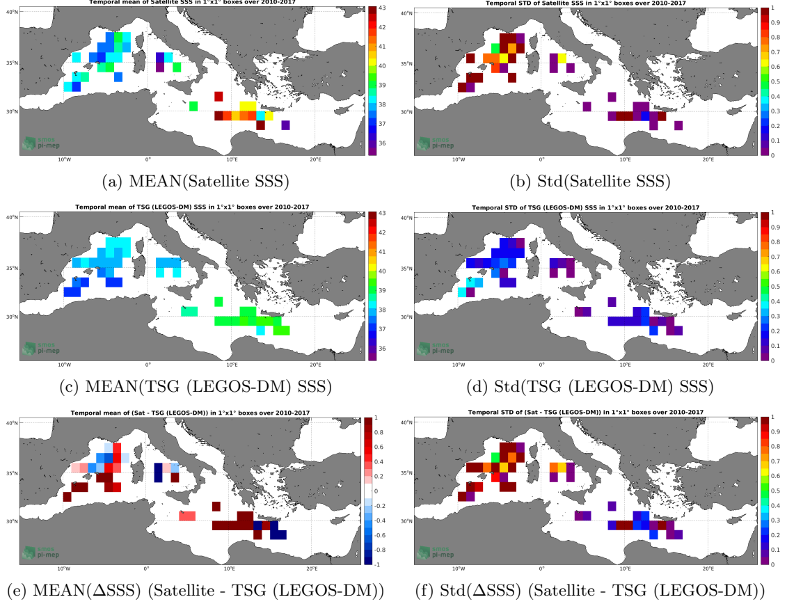
Figure 6: Temporal mean (left) and Std (right) of SSS from SMOS L4 v2 Weekly (CATDS-CECOS-IFREMER) (top), TSG (LEGOS-DM) (middle), and of \Delta SSS (Satellite - TSG (LEGOS-DM)). Only match-up pairs are used to generate these maps.
