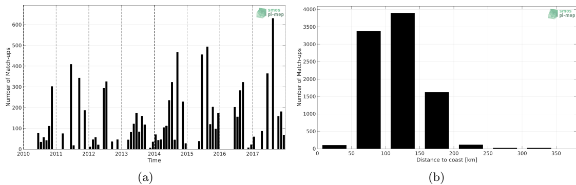
Figure 1: Number of match-ups between TSG (LEGOS-DM) and SMOS L4 v2 Weekly (CATDS-CECOS-IFREMER) SSS as a function of time (a) and as function of the distance to coast (b) over the Mediterranean Sea Pi-MEP region and for the full satellite product period.
