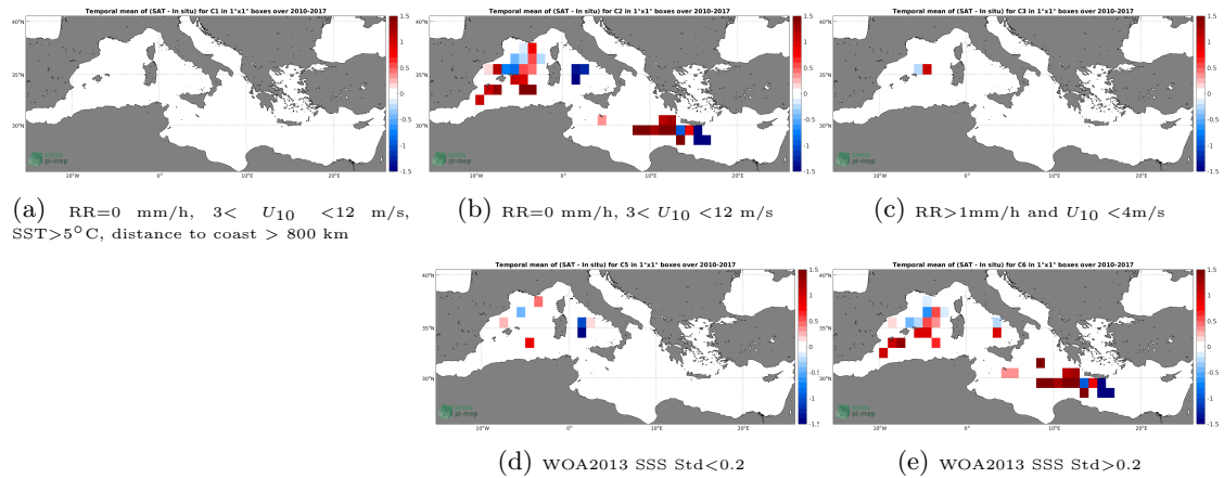
Figure 12: Temporal mean gridded over spatial boxes of size 1^{\circ}\times 1^{\circ} of \Delta\text{SSS} (SMOS L4 v2 Weekly (CATDS-CECOS-IFREMER) - TSG (LEGOS-DM)) for 5 different subdatasets corresponding to:RR=0 mm/h, 3 < U_{10} < 12 m/s, SST >5^{\circ}\text{C} , distance to coast > 800 km (a), RR=0 mm/h, 3 < U_{10} < 12 m/s (b), RR >1 mm/h and U_{10} < 4 m/s (c), WOA2013 SSS Std <0.2 (d), WOA2013 SSS Std >0.2 (e).
