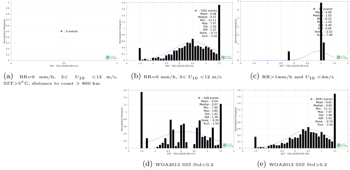
Figure 13: Normalized histogram of \Delta SSS (SMOS-L4-CATDS-CECOS-IFREMER-V2-WEEKLY-0.5DEG - TSG-LEGOS-DM) for 5 different subdatasets corresponding to: RR=0 mm/h, 3 < U_{10} < 12 m/s, SST>5°C, distance to coast > 800 km (a), RR=0 mm/h, 3 < U_{10} < 12 m/s (b), RR>1mm/h and U_{10} < 4 m/s (c), WOA2013 SSS Std<0.2 (d), WOA2013 SSS Std>0.2 (e).
