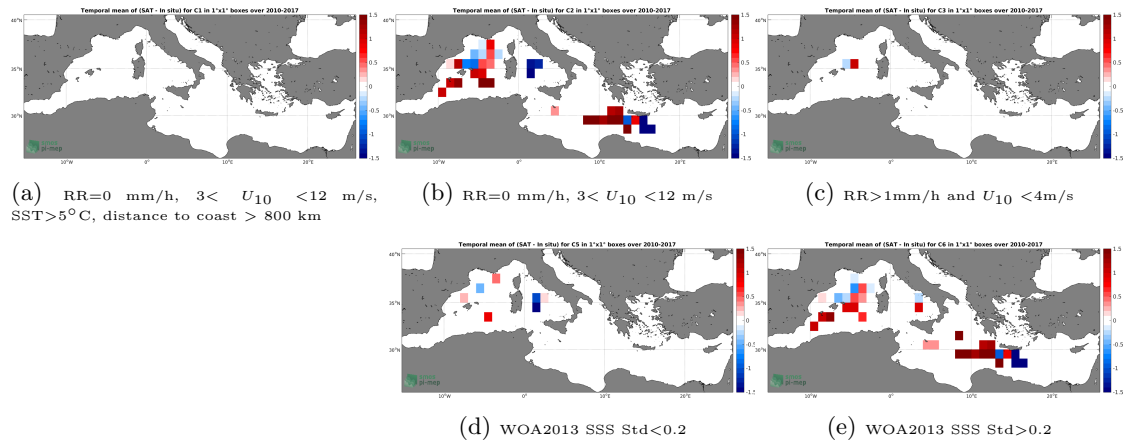
Figure 12: Temporal mean gridded over spatial boxes of size 1^{\circ}\times 1^{\circ} of \Delta\text{SSS} (SMOS-L4-CATDS-CECOS-IFREMER-V2-WEEKLY-0.5DEG - TSG-LEGOS-DM) for 5 different subdatasets corresponding to: RR=0 mm/h, 3 < U_{10} < 12 m/s, SST > 5^{\circ}\text{C} , distance to coast > 800 km (a), RR=0 mm/h, 3 < U_{10} < 12 m/s (b), RR > 1 mm/h and U_{10} < 4 m/s (c), WOA2013 SSS Std < 0.2 (d), WOA2013 SSS Std > 0.2 (e).
