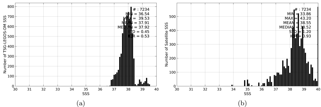
Figure 2: Histograms of SSS from TSG-LEGOS-DM (a) and SMOS-L4-CATDS-CECOS-IFREMER-V2-WEEKLY-0.5DEG (b) considering all match-up pairs per bins of 0.1 over the Mediterranean Sea Pi-MEP region and for the full satellite product period.
