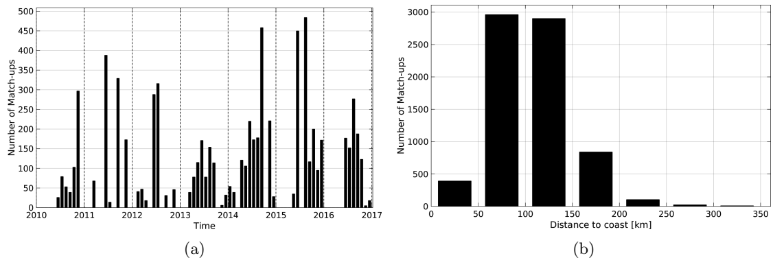
Figure 1: Number of match-ups between TSG-LEGOS-DM and SMOS-L4-CATDS-CECOS-IFREMER-V2-WEEKLY-0.5DEG SSS as a function of time (a) and as function of the distance to coast (b) over the Mediterranean Sea Pi-MEP region and for the full satellite product period.
