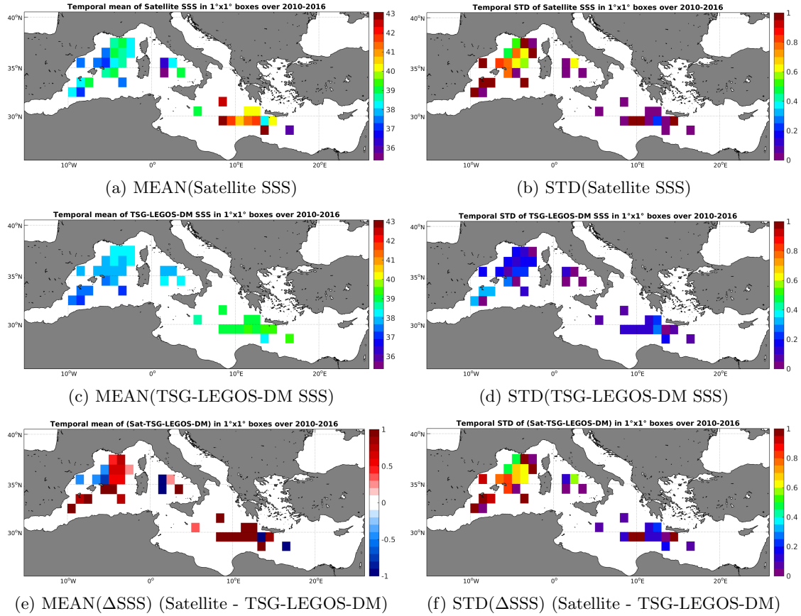
Figure 6: Temporal mean (left) and STD (right) of SSS from SMOS-L4-CATDS-CECOS-IFREMER-V2-WEEKLY-0.5DEG (top), TSG-LEGOS-DM (middle), and of \Delta SSS (Satellite - TSG-LEGOS-DM). Only match-up pairs are used to generate these maps.
