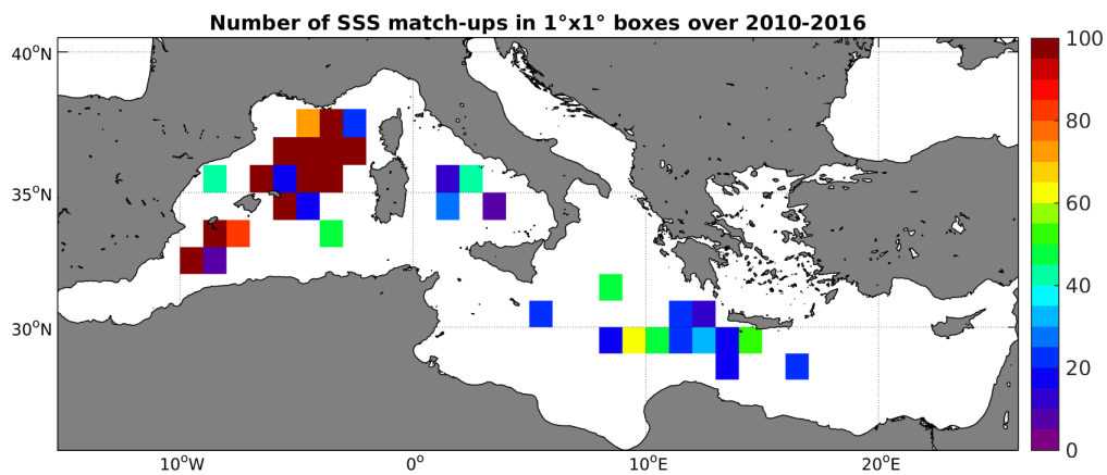
Figure 4: Number of SSS match-ups between TSG-LEGOS-DM SSS and the SMOS-L4-CATDS-CECOS-IFREMER-V2-WEEKLY-0.5DEG SSS product for the Mediterranean Sea Pi-MEP region over 1^\circ \times 1^\circ boxes and for the full satellite product period.
