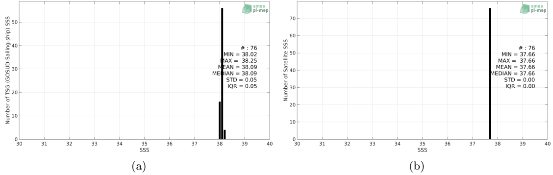
Figure 2: Histograms of SSS from TSG (GOSUD-Sailing-ship) (a) and SMOS L4 v2 Weekly (CATDS-CECOS-IFREMER) (b) considering all match-up pairs per bins of 0.1 over the Mediterranean Sea Pi-MEP region and for the full satellite product period.
