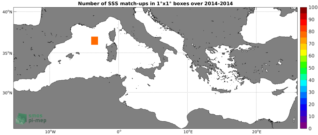
Figure 4: Number of SSS match-ups between TSG (GOSUD-Sailing-ship) SSS and the SMOS L4 v2 Weekly (CATDS-CECOS-IFREMER) SSS product for the Mediterranean Sea Pi-MEP region over 1^\circ \times 1^\circ boxes and for the full satellite product period.
