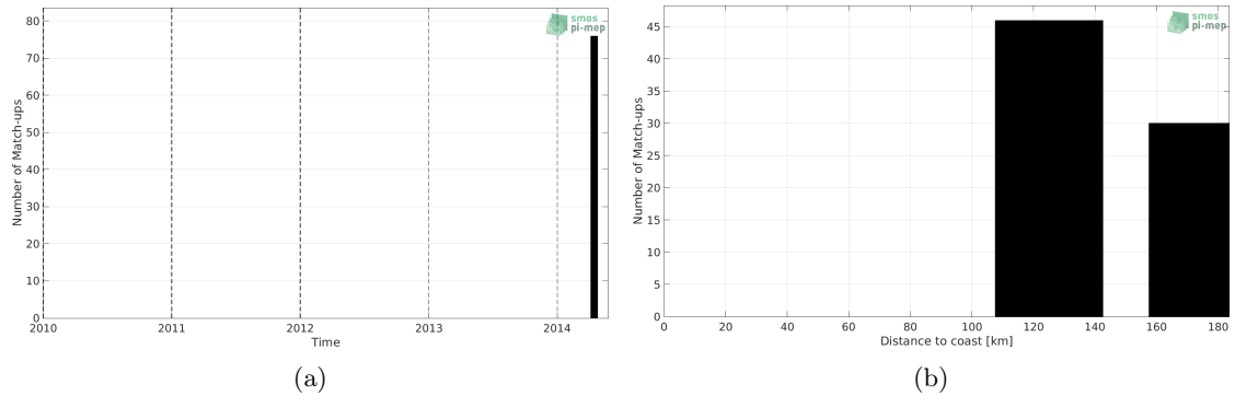
Figure 1: Number of match-ups between TSG (GOSUD-Sailing-ship) and SMOS L4 v2 Weekly (CATDS-CECOS-IFREMER) SSS as a function of time (a) and as function of the distance to coast (b) over the Mediterranean Sea Pi-MEP region and for the full satellite product period.
