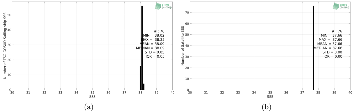
Figure 2: Histograms of SSS from TSG-GOSUD-Sailing-ship (a) and SMOS-L4-CATDS-CECOS-IFREMER-V2-WEEKLY-0.5DEG (b) considering all match-up pairs per bins of 0.1 over the Mediterranean Sea Pi-MEP region and for the full satellite product period.
