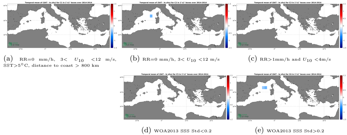
Figure 12: Temporal mean gridded over spatial boxes of size 1^{\circ}\times 1^{\circ} of \Delta SSS (SMOS-L4-CATDS-CECOS-IFREMER-V2-WEEKLY-0.5DEG - TSG-GOSUD-Sailing-ship) for 5 different subdatasets corresponding to:RR=0 mm/h, 3 < U_{10} < 12 m/s, SST >5^{\circ}\text{C} , distance to coast > 800 km (a), RR=0 mm/h, 3 < U_{10} < 12 m/s (b), RR >1 mm/h and U_{10} < 4 m/s (c), WOA2013 SSS Std <0.2 (d), WOA2013 SSS Std >0.2 (e).
