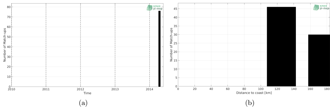
Figure 1: Number of match-ups between TSG-GOSUD-Sailing-ship and SMOS-L4-CATDS-CECOS-IFREMER-V2-WEEKLY-0.5DEG SSS as a function of time (a) and as function of the distance to coast (b) over the Mediterranean Sea Pi-MEP region and for the full satellite product period.
