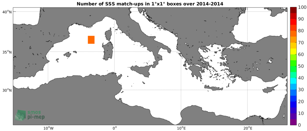
Figure 4: Number of SSS match-ups between TSG-GOSUD-Sailing-ship SSS and the SMOS-L4-CATDS-CECOS-IFREMER-V2-WEEKLY-0.5DEG SSS product for the Mediterranean Sea Pi-MEP region over 1°x1° boxes and for the full satellite product period.
