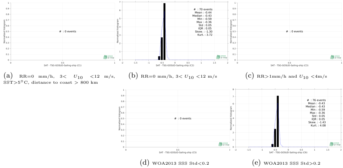
Figure 13: Normalized histogram of \Delta SSS (SMOS-L4-CATDS-CECOS-IFREMERE-V2-WEEKLY-0.5DEG - TSG-GOSUD-Sailing-ship) for 5 different subdatasets corresponding to: RR=0 mm/h, 3 < U_{10} < 12 m/s, SST>5°C, distance to coast > 800 km (a), RR=0 mm/h, 3 < U_{10} < 12 m/s (b), RR>1mm/h and U_{10} < 4 m/s (c), WOA2013 SSS Std<0.2 (d), WOA2013 SSS Std>0.2 (e).
