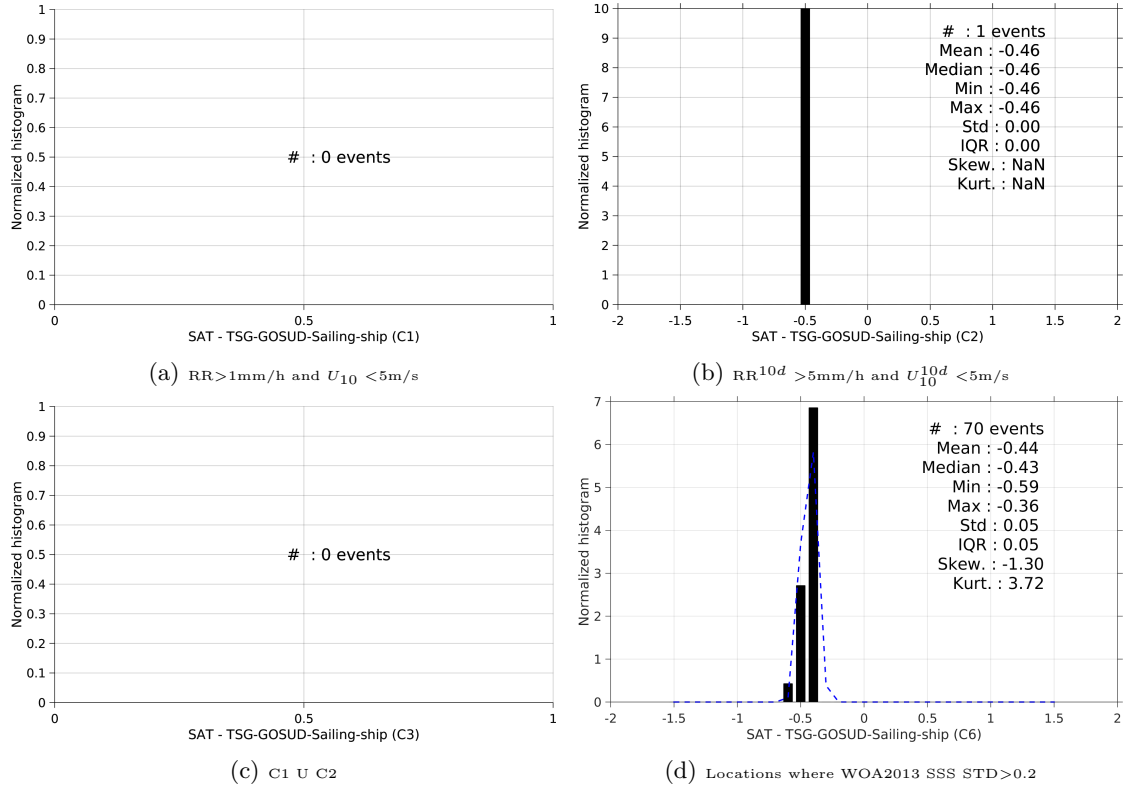
Figure 13: Normalized histogram of \Delta\text{SSS} (SMOS-L4-CATDS-CECOS-IFREMER-V2-WEEKLY-0.5DEG - TSG-GOSUD-Sailing-ship) for 6 different subdatasets corresponding to: RR > 1\text{mm/h} and U_{10} < 5\text{m/s} (a), RR^{10d} > 5\text{mm/h} and U_{10}^{10d} < 5\text{m/s} (b), C1 U C2 (c), Locations where WOA2013 SSS STD > 0.2 (d).
