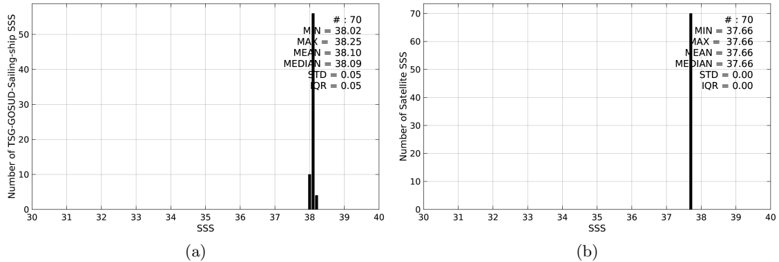
Figure 2: Histograms of SSS from TSG-GOSUD-Sailing-ship (a) and SMOS-L4-CATDS-CECOS-IFREMER-V2-WEEKLY-0.5DEG (b) considering all match-up pairs per bins of 0.1 over the Mediterranean Sea Pi-MEP region and for the full satellite product period.
