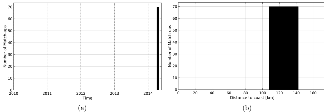
Figure 1: Number of match-ups between TSG-GOSUD-Sailing-ship and SMOS-L4-CATDS-CECOS-IFREMER-V2-WEEKLY-0.5DEG SSS as a function of time (a) and as function of the distance to coast (b) over the Mediterranean Sea Pi-MEP region and for the full satellite product period.
