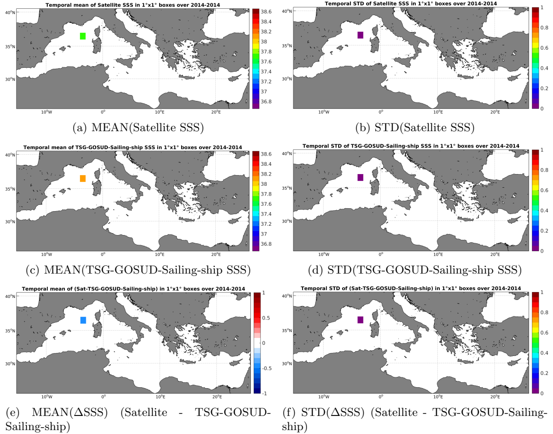
Figure 6: Temporal mean (left) and STD (right) of SSS from SMOS-L4-CATDS-CECOS-IFREMER-V2-WEEKLY-0.5DEG (top), TSG-GOSUD-Sailing-ship (middle), and of \Delta\text{SSS} (Satellite - TSG-GOSUD-Sailing-ship). Only match-up pairs are used to generate these maps.
