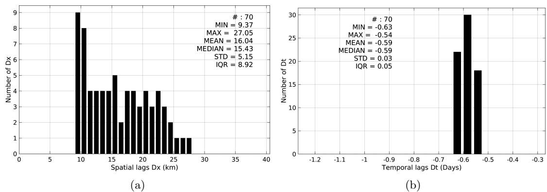
Figure 5: Histograms of the spatial (a) and temporal (b) lags between the time of the TSG-GOSUD-Sailing-ship measurements and the date of the corresponding SMOS-L4-CATDS-CECOS-IFREMER-V2-WEEKLY-0.5DEG SSS product.
