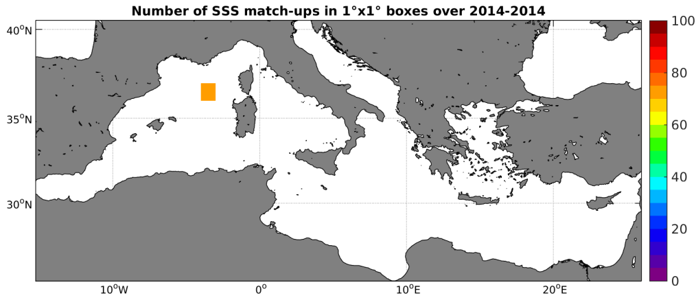
Figure 4: Number of SSS match-ups between TSG-GOSUD-Sailing-ship SSS and the SMOS-L4-CATDS-CECOS-IFREMER-V2-WEEKLY-0.5DEG SSS product for the Mediterranean Sea Pi-MEP region over 1^\circ \times 1^\circ boxes and for the full satellite product period.
