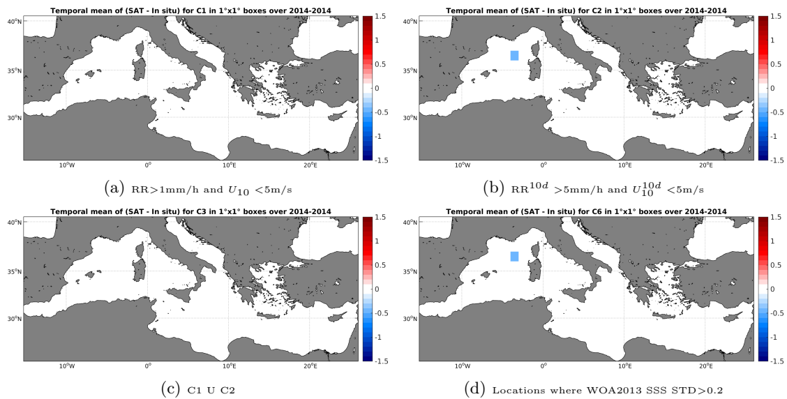
Figure 12: Temporal mean gridded over spatial boxes of size 1^\circ \times 1^\circ of \Delta SSS (SMOS-L4-CATDS-CECOS-IFREMER-V2-WEEKLY-0.5DEG - TSG-GOSUD-Sailing-ship) for 4 different subdatasets corresponding to: RR > 1\text{mm/h} and U_{10} < 5\text{m/s} (a), RR^{10d} > 5\text{mm/h} and U_{10}^{10d} < 5\text{m/s} (b), C1 U C2 (c), Locations where WOA2013 SSS STD > 0.2 (d).
