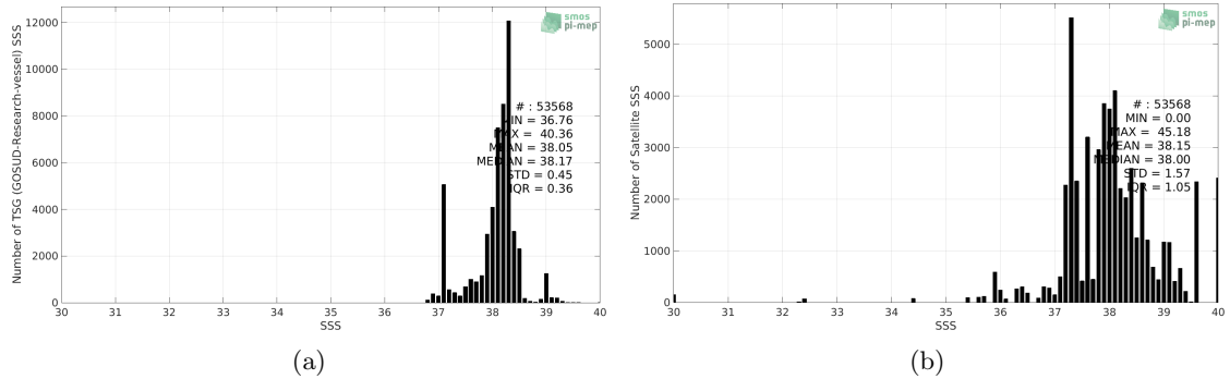
Figure 2: Histograms of SSS from TSG (GOSUD-Research-vessel) (a) and SMOS L4 v2 Weekly (CATDS-CECOS-IFREMER) (b) considering all match-up pairs per bins of 0.1 over the Mediterranean Sea Pi-MEP region and for the full satellite product period.
