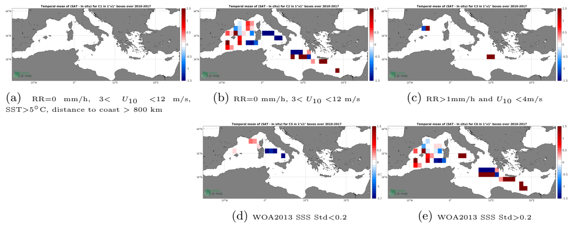
Figure 12: Temporal mean gridded over spatial boxes of size 1^\circ \times 1^\circ of \Delta SSS (SMOS-L4-CATDS-CECOS-IFREMER-V2-WEEKLY-0.5DEG - TSG-GOSUD-Research-vessel) for 5 different sub-datasets corresponding to:RR=0 mm/h, 3 < U_{10} < 12 m/s, SST >5^\circ\text{C} , distance to coast > 800 km (a), RR=0 mm/h, 3 < U_{10} < 12 m/s (b), RR >1 mm/h and U_{10} < 4 m/s (c), WOA2013 SSS Std <0.2 (d), WOA2013 SSS Std >0.2 (e).
