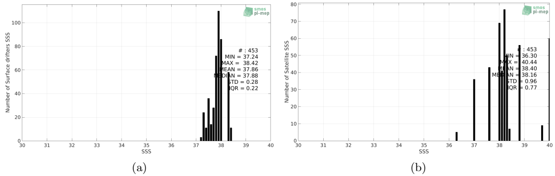
Figure 2: Histograms of SSS from Surface drifters (a) and SMOS L4 v2 Weekly (CATDS-CECOS-IFREMER) (b) considering all match-up pairs per bins of 0.1 over the Mediterranean Sea Pi-MEP region and for the full satellite product period.
