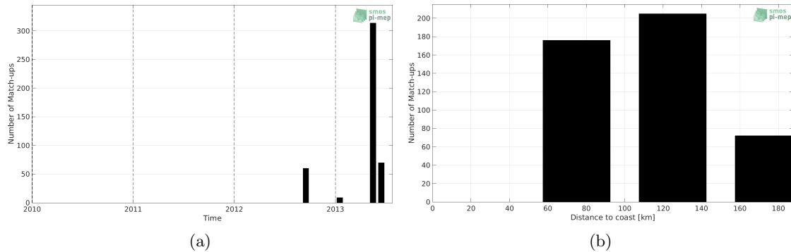
Figure 1: Number of match-ups between Surface drifters and SMOS L4 v2 Weekly (CATDS-CECOS-IFREMER) SSS as a function of time (a) and as function of the distance to coast (b) over the Mediterranean Sea Pi-MEP region and for the full satellite product period.
