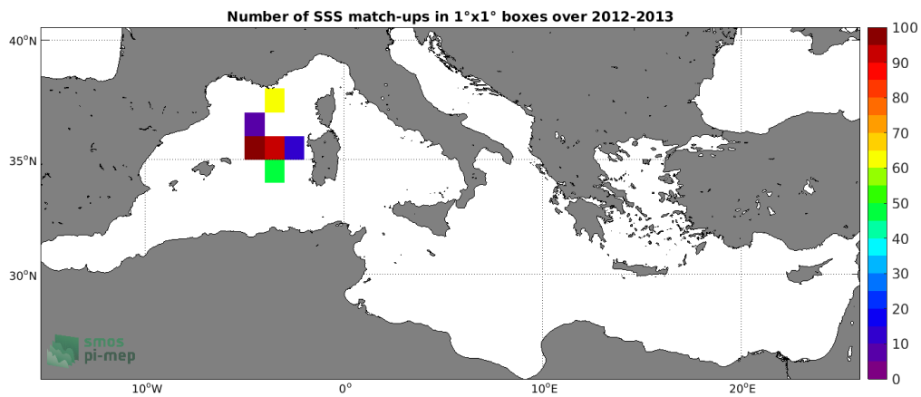
Figure 3: Number of SSS match-ups between Surface drifters SSS and the SMOS L4 v2 Weekly (CATDS-CECOS-IFREMER) SSS product for the Mediterranean Sea Pi-MEP region over 1^\circ \times 1^\circ boxes and for the full satellite product period.
