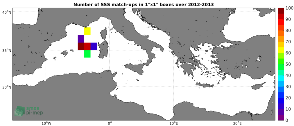
Figure 3: Number of SSS match-ups between Surface drifters SSS and the SMOS-L4-CATDS-CECOS-IFREMER-V2-WEEKLY-0.5DEG SSS product for the Mediterranean Sea Pi-MEP region over 1°x1° boxes and for the full satellite product period.
