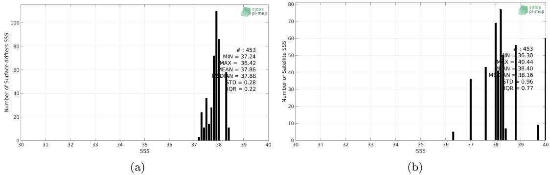
Figure 2: Histograms of SSS from Surface drifters (a) and SMOS-L4-CATDS-CECOS-IFREMER-V2-WEEKLY-0.5DEG (b) considering all match-up pairs per bins of 0.1 over the Mediterranean Sea Pi-MEP region and for the full satellite product period.
