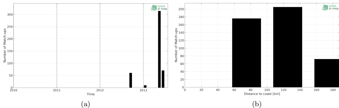
Figure 1: Number of match-ups between Surface drifters and SMOS-L4-CATDS-CECOS-IFREMER-V2-WEEKLY-0.5DEG SSS as a function of time (a) and as function of the distance to coast (b) over the Mediterranean Sea Pi-MEP region and for the full satellite product period.
