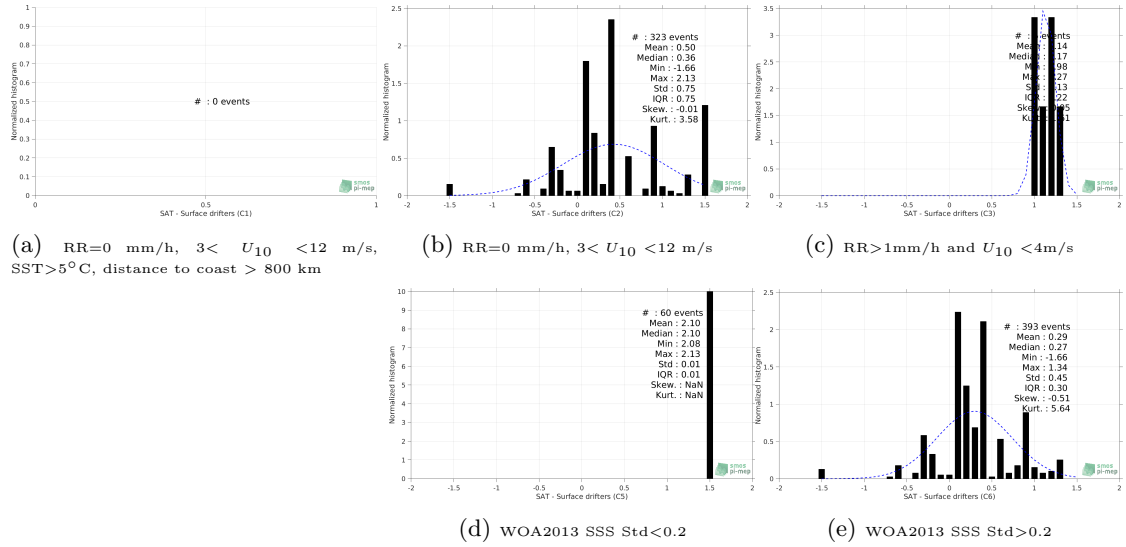
Figure 12: Normalized histogram of \Delta SSS (SMOS-L4-CATDS-CECOS-IFREMER-V2-WEEKLY-0.5DEG - Surface drifters) for 5 different subdatasets corresponding to: RR=0 mm/h, 3 < U_{10} < 12 m/s, SST > 5°C, distance to coast > 800 km (a), RR=0 mm/h, 3 < U_{10} < 12 m/s (b), RR > 1mm/h and U_{10} < 4 m/s (c), WOA2013 SSS Std < 0.2 (d), WOA2013 SSS Std > 0.2 (e).
