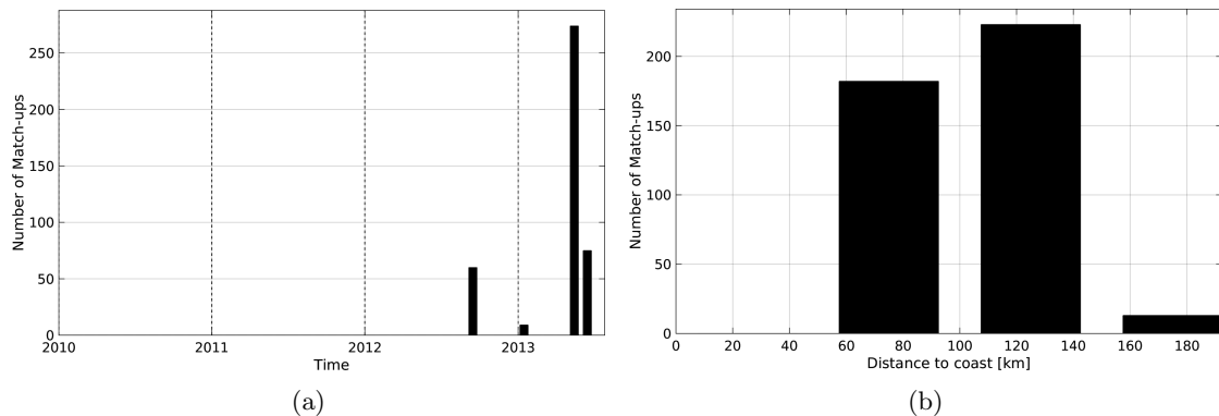
Figure 1: Number of match-ups between Surface drifters and SMOS-L4-CATDS-CECOS-IFREMER-V2-WEEKLY-0.5DEG SSS as a function of time (a) and as function of the distance to coast (b) over the Mediterranean Sea Pi-MEP region and for the full satellite product period.
