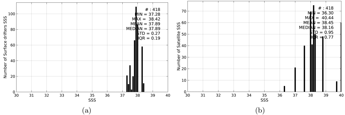
Figure 2: Histograms of SSS from Surface drifters (a) and SMOS-L4-CATDS-CECOS-IFREMER-V2-WEEKLY-0.5DEG (b) considering all match-up pairs per bins of 0.1 over the Mediterranean Sea Pi-MEP region and for the full satellite product period.
