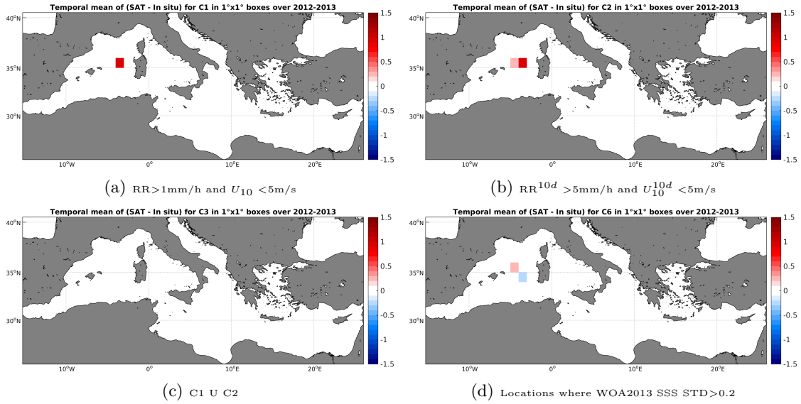
Figure 11: Temporal mean gridded over spatial boxes of size 1°x1° of \Delta SSS (SMOS-L4-CATDS-CECOS-IFREMER-V2-WEEKLY-0.5DEG - Surface drifters) for 4 different subdatasets corresponding to:RR>1mm/h and U_{10} < 5 m/s (a), RR^{10d} > 5 mm/h and U_{10}^{10d} < 5 m/s (b), C1 U C2 (c),Locations where WOA2013 SSS STD>0.2 (d).
