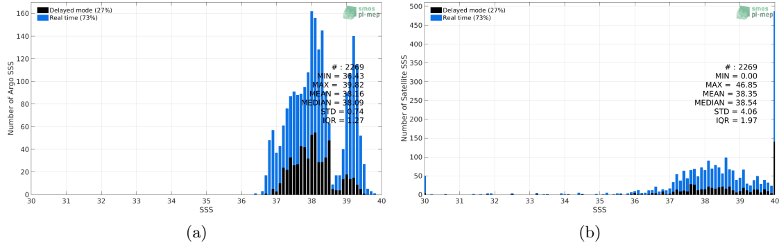
Figure 2: Histograms of SSS from Argo (a) and SMOS L4 v2 Weekly (CATDS-CECOS-IFREMER) (b) considering all match-up pairs per bins of 0.1 over the Mediterranean Sea Pi-MEP region and for the full satellite product period.
