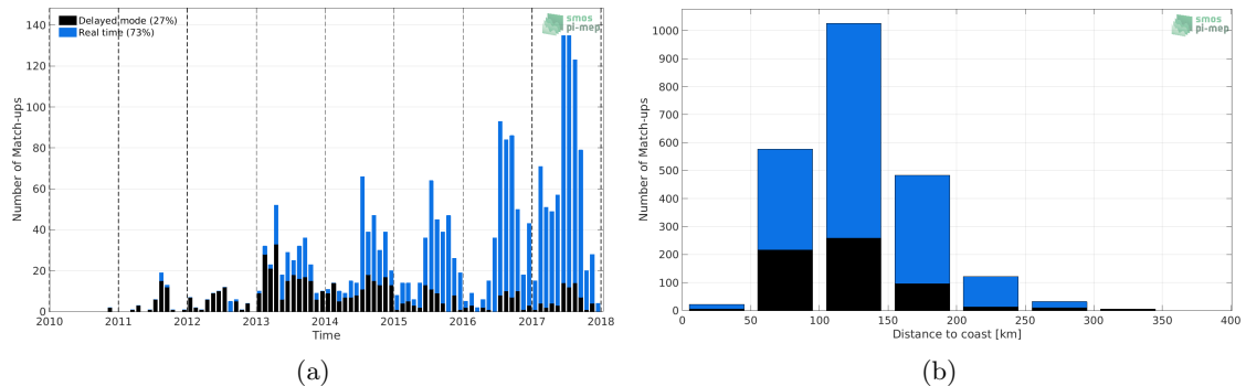
Figure 1: Number of match-ups between Argo and SMOS L4 v2 Weekly (CATDS-CECOS-IFREMER) SSS as a function of time (a) and as function of the distance to coast (b) over the Mediterranean Sea Pi-MEP region and for the full satellite product period.
