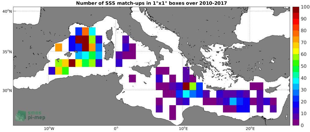
Figure 4: Number of SSS match-ups between Argo SSS and the SMOS L4 v2 Weekly (CATDS-CECOS-IFREMER) SSS product for the Mediterranean Sea Pi-MEP region over 1^\circ \times 1^\circ boxes and for the full satellite product period.
