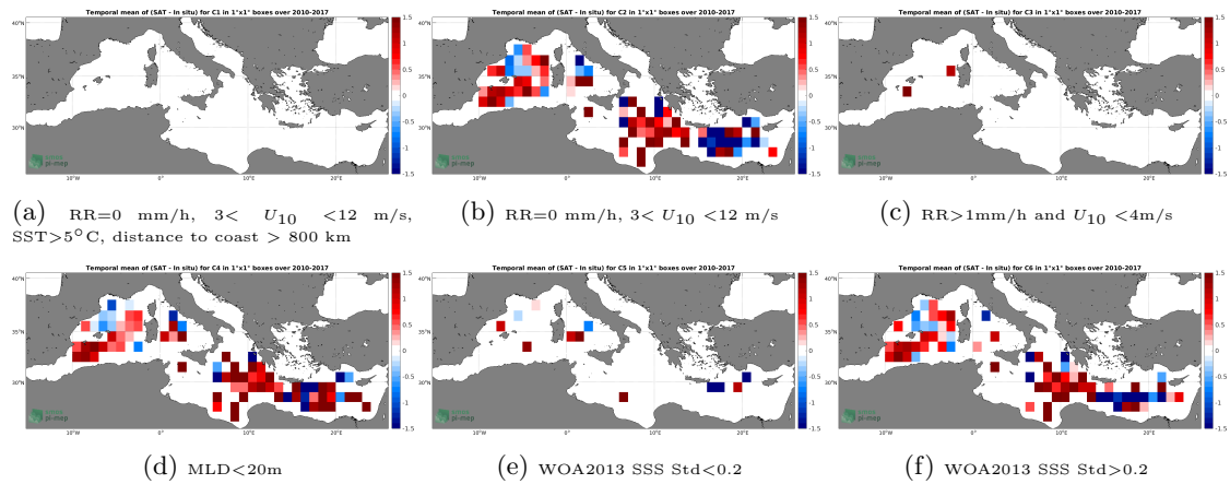
Figure 12: Temporal mean gridded over spatial boxes of size 1^\circ \times 1^\circ of \Delta SSS (SMOS L4 v2 Weekly (CATDS-CECOS-IFREMER) - Argo) for 6 different subdatasets corresponding to:RR=0 mm/h, 3 < U_{10} < 12 m/s, SST >5^\circ\text{C} , distance to coast > 800 km (a), RR=0 mm/h, 3 < U_{10} < 12 m/s (b), RR >1 mm/h and U_{10} < 4 m/s (c),MLD <20 m (d),WOA2013 SSS Std <0.2 (e),WOA2013 SSS Std >0.2 (f).
