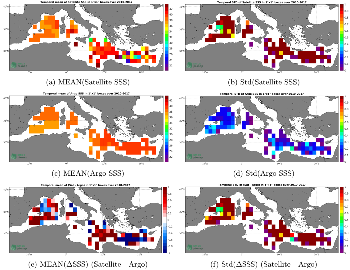
Figure 6: Temporal mean (left) and Std (right) of SSS from SMOS L4 v2 Weekly (CATDS-CECOS-IFREMER) (top), Argo (middle), and of \Delta SSS (Satellite - Argo). Only match-up pairs are used to generate these maps.
