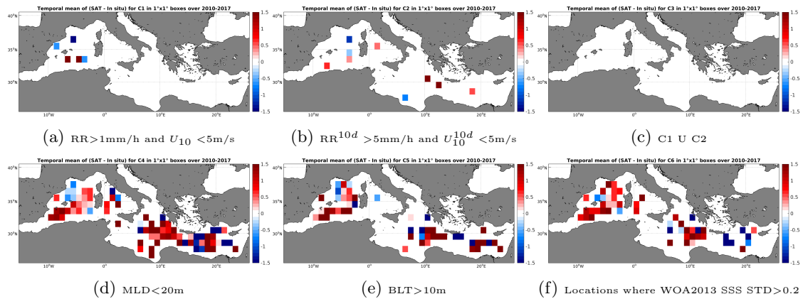
Figure 12: Temporal mean gridded over spatial boxes of size 1^\circ \times 1^\circ of \Delta SSS (SMOS-L4-CATDS-CECOS-IFREMER-V2-WEEKLY-0.5DEG - Argo) for 6 different subdatasets corresponding to:RR >1 mm/h and U_{10} < 5 m/s (a), RR ^{10d} > 5 mm/h and U_{10}^{10d} < 5 m/s (b), C1 U C2 (c),MLD <20 m (d),BLT >10 m (e),Locations where WOA2013 SSS STD >0.2 (f).
