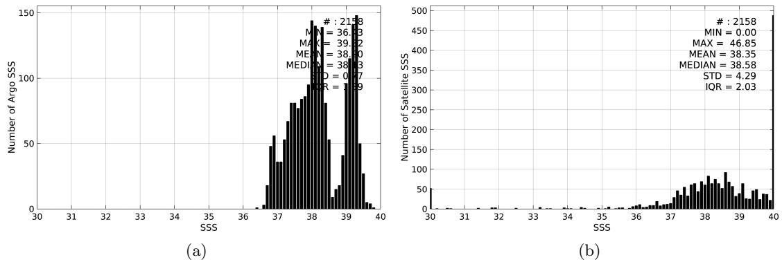
Figure 2: Histograms of SSS from Argo (a) and SMOS-L4-CATDS-CECOS-IFREMER-V2-WEEKLY-0.5DEG (b) considering all match-up pairs per bins of 0.1 over the Mediterranean Sea Pi-MEP region and for the full satellite product period.
