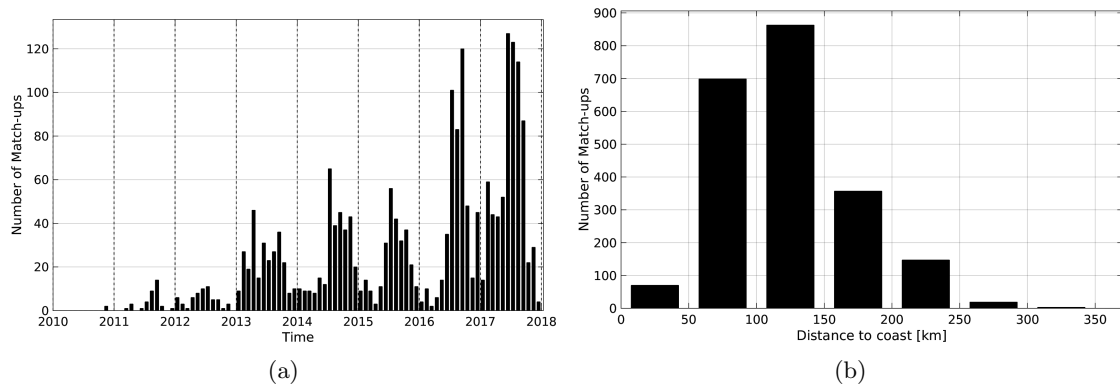
Figure 1: Number of match-ups between Argo and SMOS-L4-CATDS-CECOS-IFREMER-V2-WEEKLY-0.5DEG SSS as a function of time (a) and as function of the distance to coast (b) over the Mediterranean Sea Pi-MEP region and for the full satellite product period.
