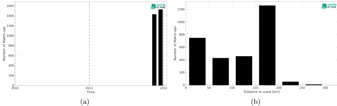
Figure 2: Number of match-ups between TSG (SAMOS) and SMOS SSS L4 v2 - Daily (BEC) SSS as a function of time (a) and as function of the distance to coast (b) over the Mediterranean Sea Pi-MEP region and for the full satellite product period.
