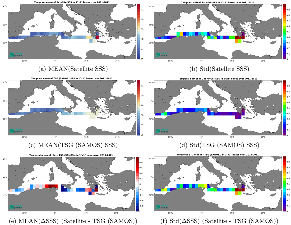
Figure 7: Temporal mean (left) and Std (right) of SSS from SMOS SSS L4 v2 - Daily (BEC) (top), TSG (SAMOS) (middle), and of \Delta\text{SSS} (Satellite - TSG (SAMOS)). Only match-up pairs are used to generate these maps.
