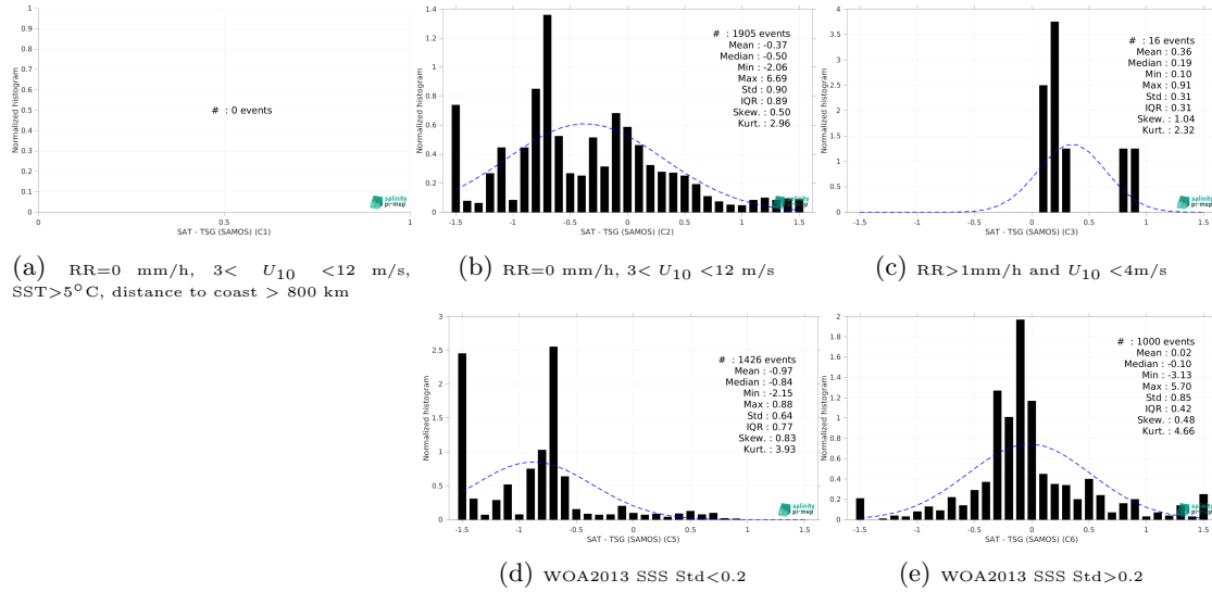
Figure 15: Normalized histogram of \Delta SSS (SMOS SSS L4 v2 - Daily (BEC) - TSG (SAMOS)) for 5 different subdatasets corresponding to: RR=0 mm/h, 3 < U_{10} < 12 m/s, SST > 5°C, distance to coast > 800 km (a), RR=0 mm/h, 3 < U_{10} < 12 m/s (b), RR > 1mm/h and U_{10} < 4 m/s (c), WOA2013 SSS Std < 0.2 (d), WOA2013 SSS Std > 0.2 (e).
