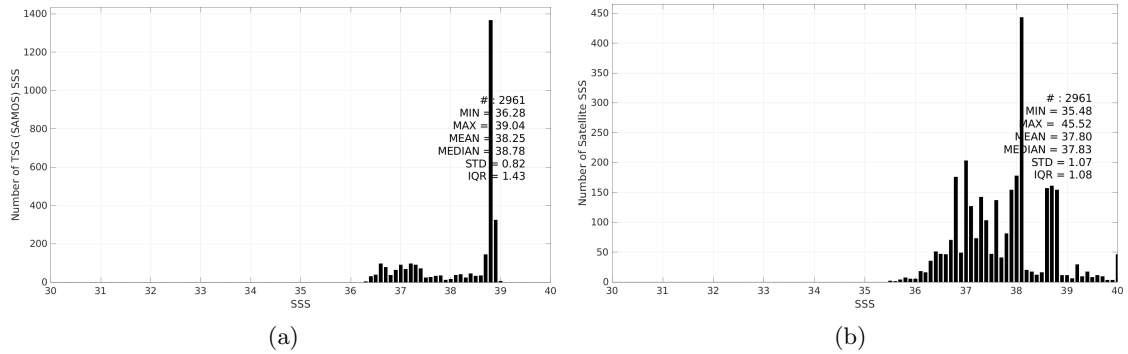
Figure 3: Histograms of SSS from TSG (SAMOS) (a) and SMOS SSS L4 v2 - Daily (BEC) (b) considering all match-up pairs per bins of 0.1 over the Mediterranean Sea Pi-MEP region and for the full satellite product period.
