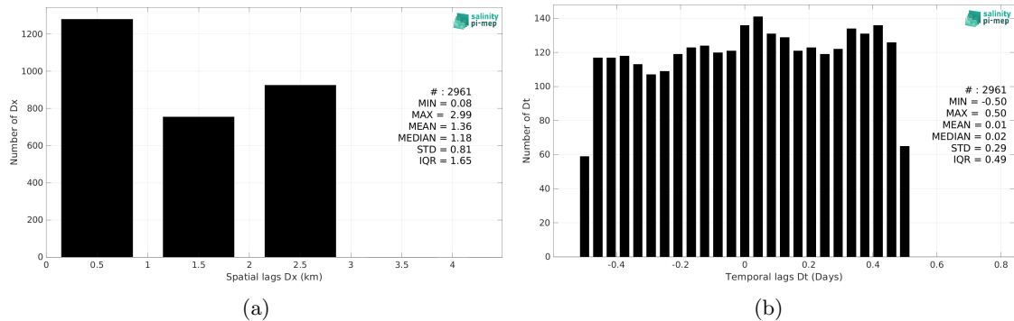
Figure 6: Histograms of the spatial (a) and temporal (b) lags between the location/time of the TSG (SAMOS) measurement and the date of the corresponding SMOS SSS L4 v2 - Daily (BEC) SSS pixel.
