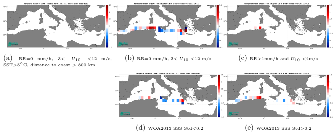
Figure 14: Temporal mean gridded over spatial boxes of size 1^\circ \times 1^\circ of \Delta SSS (SMOS SSS L4 v2 - Daily (BEC) - TSG (SAMOS)) for 5 different subdatasets corresponding to:RR=0 mm/h, 3 < U_{10} < 12 m/s, SST>5°C, distance to coast > 800 km (a), RR=0 mm/h, 3 < U_{10} < 12 m/s (b), RR>1mm/h and U_{10} < 4 m/s (c), WOA2013 SSS Std<0.2 (d), WOA2013 SSS Std>0.2 (e).
