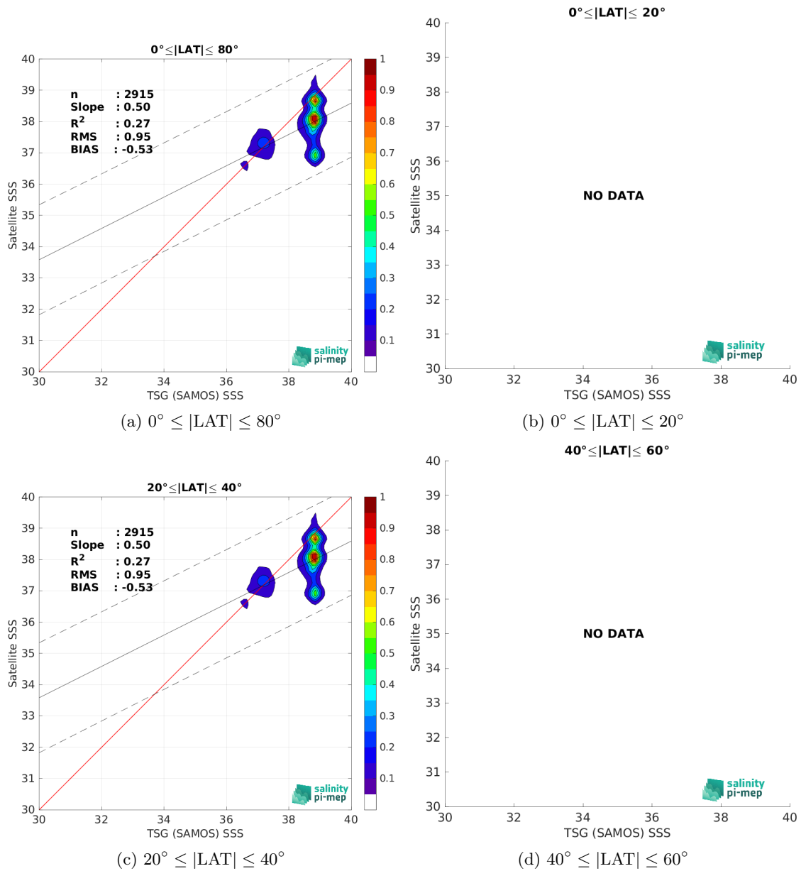
Figure 10: Contour maps of the concentration of SMOS SSS L4 v2 - Daily (BEC) SSS (y-axis) versus TSG (SAMOS) SSS (x-axis) at match-up pairs for different latitude bands. For each plot, the red line shows x=y . The black thin and dashed lines indicate a linear fit through the data cloud and the \pm 95\% confidence levels, respectively. The number match-up pairs n , the slope and R^2 coefficient of the linear fit, the root mean square (RMS) and the mean bias between satellite and in situ data are indicated for each latitude band in each plot.
