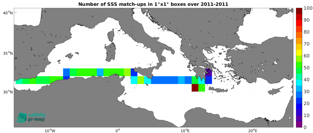
Figure 5: Number of SSS match-ups between TSG (SAMOS) SSS and the SMOS SSS L4 v2 - Daily (BEC) SSS product for the Mediterranean Sea Pi-MEP region over 1^\circ \times 1^\circ boxes and for the full satellite product period.
