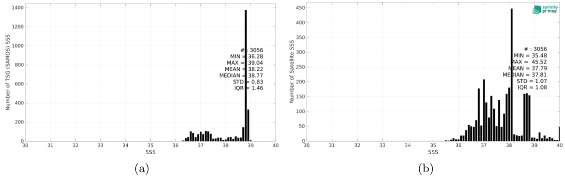
Figure 2: Histograms of SSS from TSG (SAMOS) (a) and SMOS SSS L4 v2 - Daily (BEC) (b) considering all match-up pairs per bins of 0.1 over the Mediterranean Sea Pi-MEP region and for the full satellite product period.
