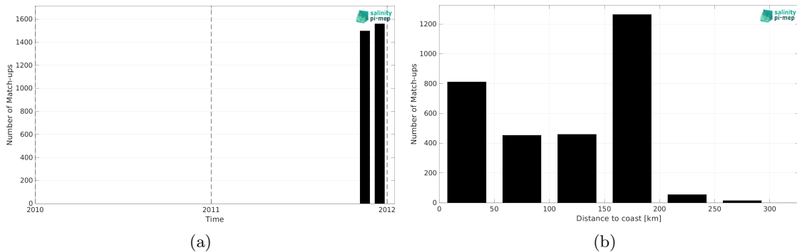
Figure 1: Number of match-ups between TSG (SAMOS) and SMOS SSS L4 v2 - Daily (BEC) SSS as a function of time (a) and as function of the distance to coast (b) over the Mediterranean Sea Pi-MEP region and for the full satellite product period.
