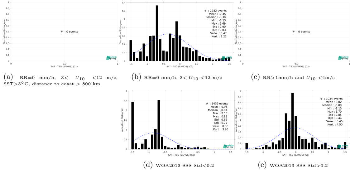
Figure 13: Normalized histogram of \Delta SSS (SMOS SSS L4 v2 - Daily (BEC) - TSG (SAMOS)) for 5 different subdatasets corresponding to: RR=0 mm/h, 3 < U_{10} < 12 m/s, SST > 5°C, distance to coast > 800 km (a), RR=0 mm/h, 3 < U_{10} < 12 m/s (b), RR > 1mm/h and U_{10} < 4 m/s (c), WOA2013 SSS Std < 0.2 (d), WOA2013 SSS Std > 0.2 (e).
