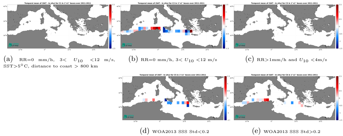
Figure 12: Temporal mean gridded over spatial boxes of size 1^{\circ}\times 1^{\circ} of \Delta\text{SSS} (SMOS SSS L4 v2 - Daily (BEC) - TSG (SAMOS)) for 5 different subdatasets corresponding to:RR=0 mm/h, 3 < U_{10} < 12 m/s, SST > 5^{\circ}\text{C} , distance to coast > 800 km (a), RR=0 mm/h, 3 < U_{10} < 12 m/s (b), RR > 1 mm/h and U_{10} < 4 m/s (c), WOA2013 SSS Std < 0.2 (d), WOA2013 SSS Std > 0.2 (e).
