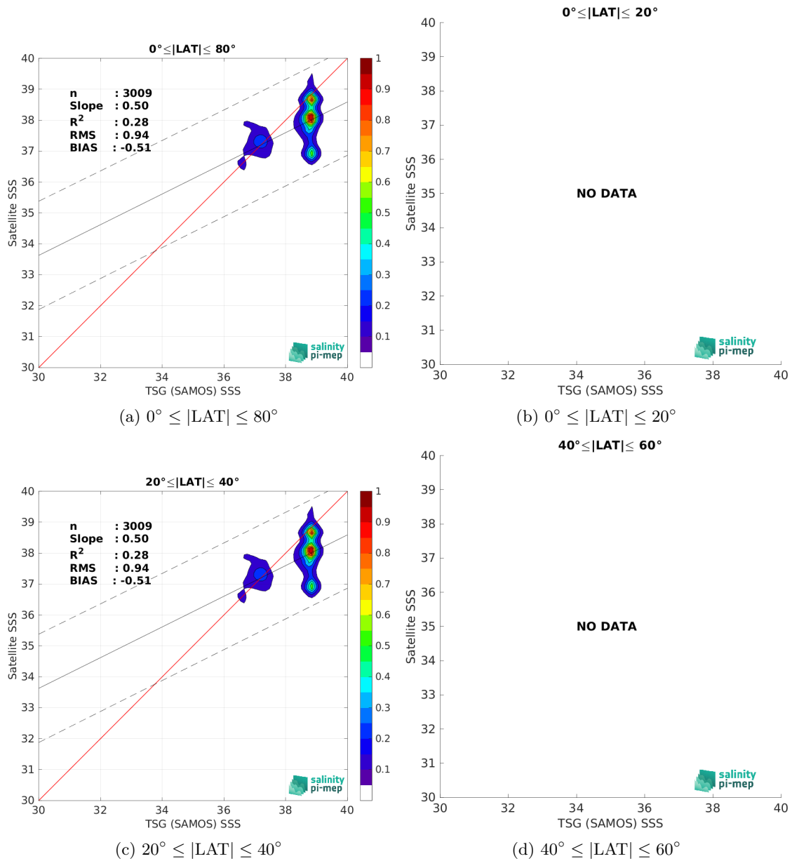
Figure 9: Contour maps of the concentration of SMOS SSS L4 v2 - Daily (BEC) SSS (y-axis) versus TSG (SAMOS) SSS (x-axis) at match-up pairs for different latitude bands. For each plot, the red line shows x=y . The black thin and dashed lines indicate a linear fit through the data cloud and the \pm 95\% confidence levels, respectively. The number match-up pairs n , the slope and R^2 coefficient of the linear fit, the root mean square (RMS) and the mean bias between satellite and in situ data are indicated for each latitude band in each plot.
