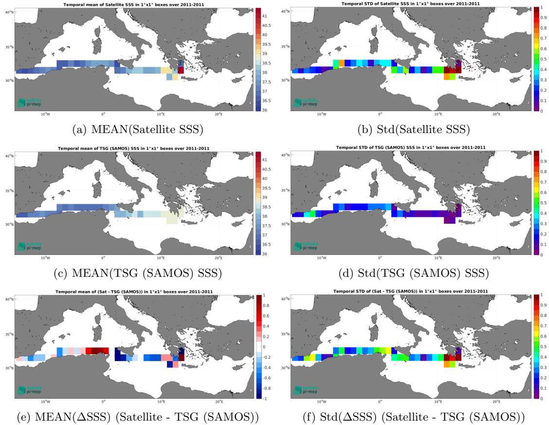
Figure 6: Temporal mean (left) and Std (right) of SSS from SMOS SSS L4 v2 - Daily (BEC) (top), TSG (SAMOS) (middle), and of \Delta\text{SSS} (Satellite - TSG (SAMOS)). Only match-up pairs are used to generate these maps.
