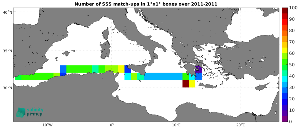
Figure 4: Number of SSS match-ups between TSG (SAMOS) SSS and the SMOS SSS L4 v2 - Daily (BEC) SSS product for the Mediterranean Sea Pi-MEP region over 1^\circ \times 1^\circ boxes and for the full satellite product period.
