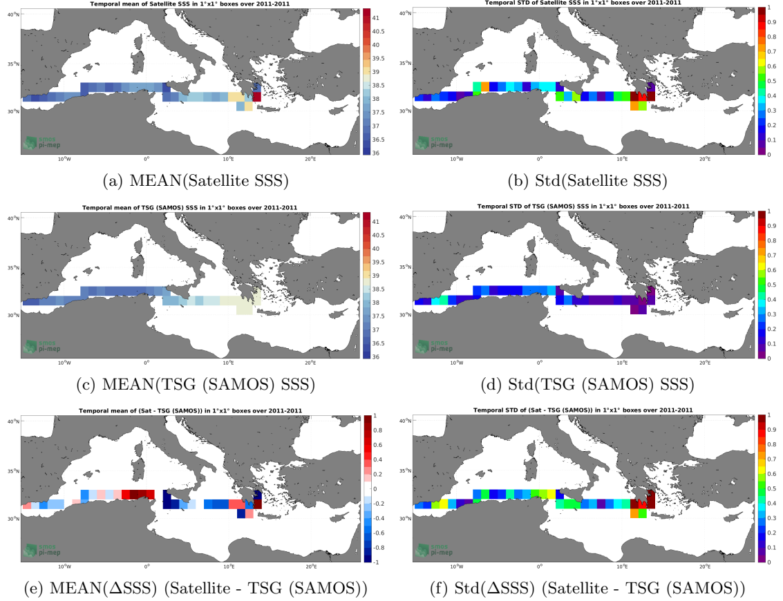
Figure 6: Temporal mean (left) and Std (right) of SSS from SMOS SSS L4 v2 - Daily (BEC) (top), TSG (SAMOS) (middle), and of \Delta\text{SSS}(\text{Satellite} - \text{TSG}(\text{SAMOS})) . Only match-up pairs are used to generate these maps.
