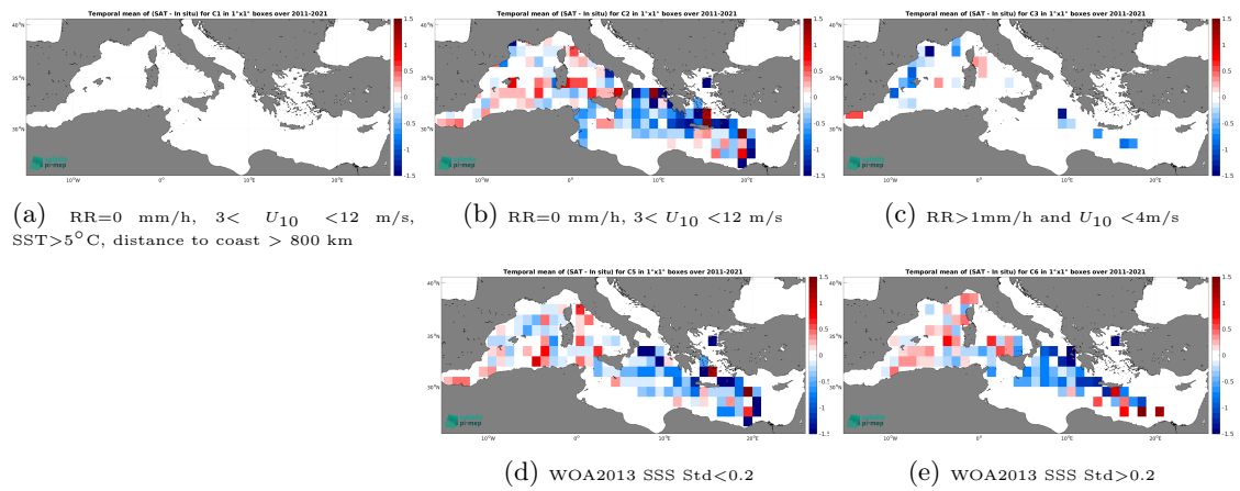
Figure 12: Temporal mean gridded over spatial boxes of size 1^\circ \times 1^\circ of \Delta SSS (SMOS SSS L4 v2 - Daily (BEC) - TSG (GOSUD-Research-vessel)) for 5 different subdatasets corresponding to:RR=0 mm/h, 3 < U_{10} < 12 m/s, SST>5°C, distance to coast > 800 km (a), RR=0 mm/h, 3 < U_{10} < 12 m/s (b), RR>1mm/h and U_{10} < 4 m/s (c), WOA2013 SSS Std<0.2 (d), WOA2013 SSS Std>0.2 (e).
