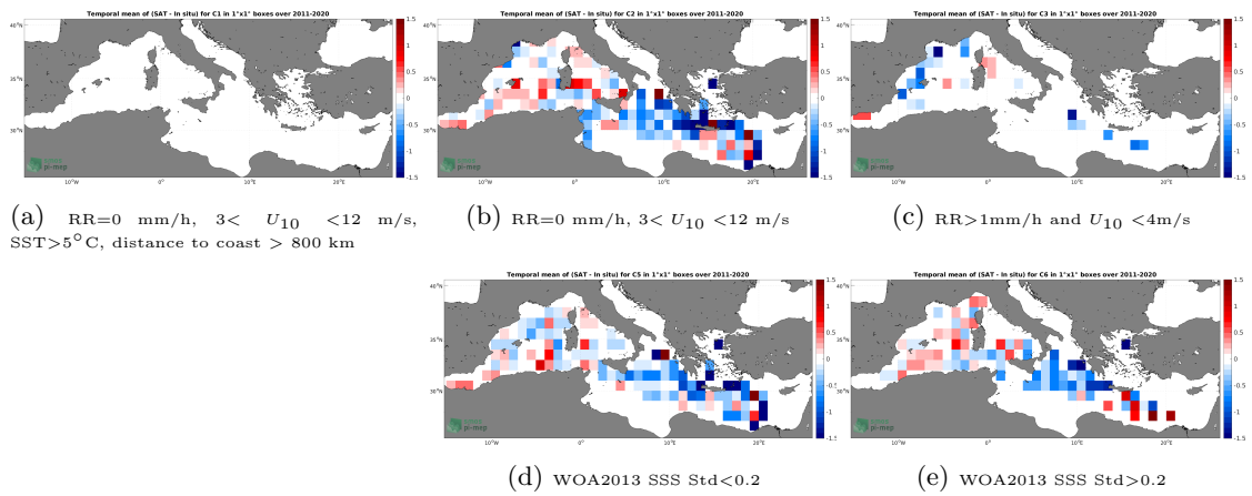
Figure 12: Temporal mean gridded over spatial boxes of size 1^\circ \times 1^\circ of \Delta SSS (SMOS SSS L4 v2 - Daily (BEC) - TSG (GOSUD-Research-vessel)) for 5 different subdatasets corresponding to:RR=0 mm/h, 3 < U_{10} < 12 m/s, SST>5°C, distance to coast > 800 km (a), RR=0 mm/h, 3 < U_{10} < 12 m/s (b), RR>1mm/h and U_{10} < 4 m/s (c), WOA2013 SSS Std<0.2 (d), WOA2013 SSS Std>0.2 (e).
