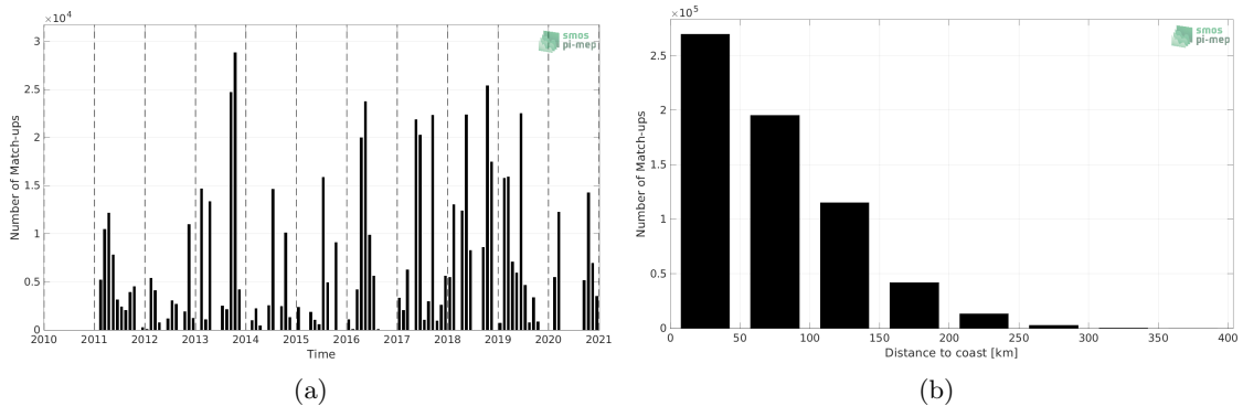
Figure 1: Number of match-ups between TSG (GOSUD-Research-vessel) and SMOS SSS L4 v2 - Daily (BEC) SSS as a function of time (a) and as function of the distance to coast (b) over the Mediterranean Sea Pi-MEP region and for the full satellite product period.
