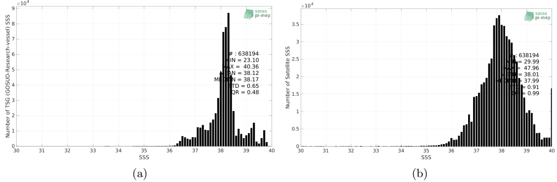
Figure 2: Histograms of SSS from TSG (GOSUD-Research-vessel) (a) and SMOS SSS L4 v2 - Daily (BEC) (b) considering all match-up pairs per bins of 0.1 over the Mediterranean Sea Pi-MEP region and for the full satellite product period.
