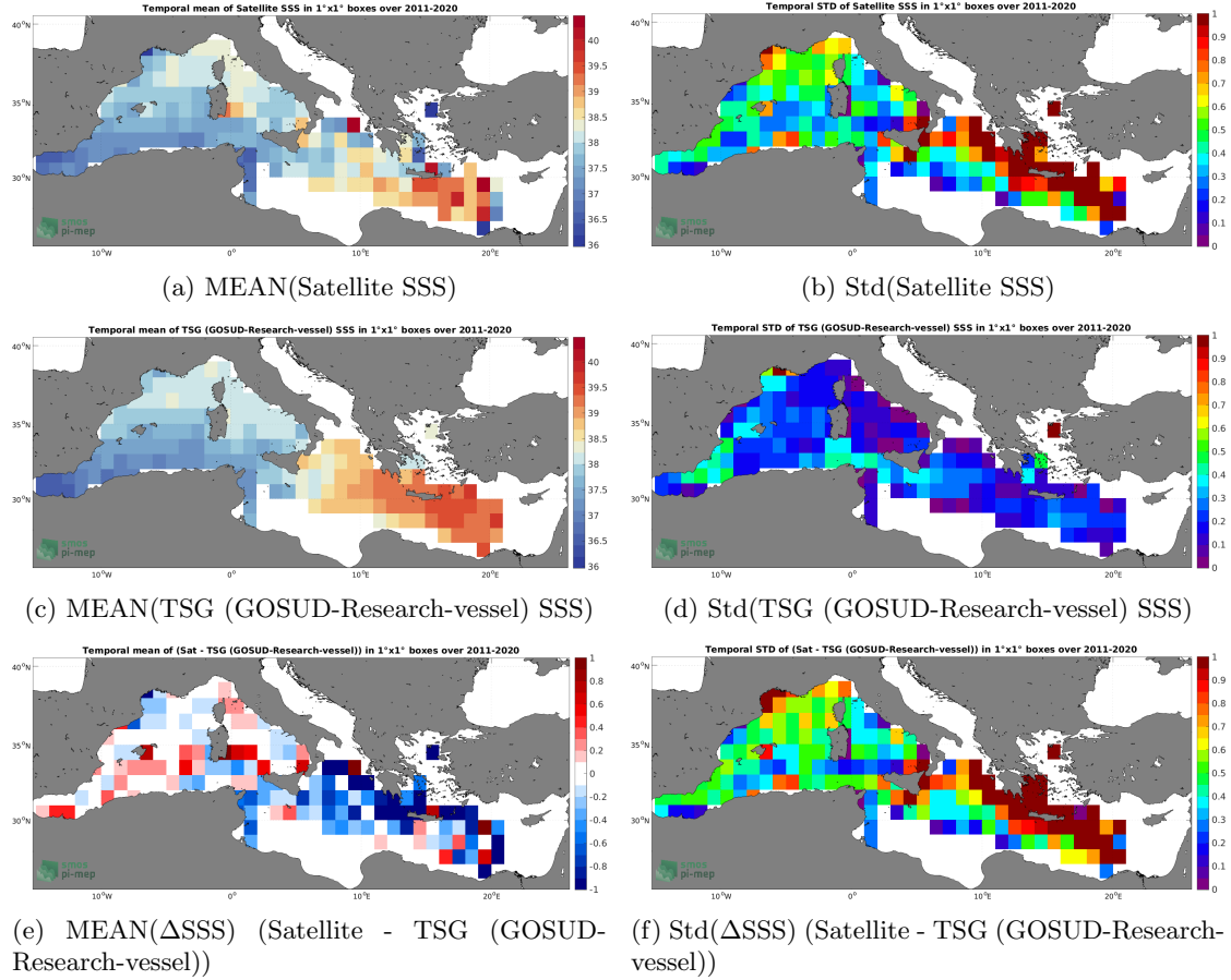
Figure 6: Temporal mean (left) and Std (right) of SSS from SMOS SSS L4 v2 - Daily (BEC) (top), TSG (GOSUD-Research-vessel) (middle), and of \Delta\text{SSS} (Satellite - TSG (GOSUD-Research-vessel)). Only match-up pairs are used to generate these maps.
