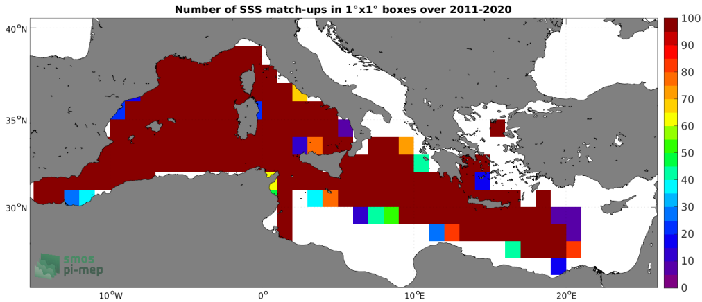
Figure 4: Number of SSS match-ups between TSG (GOSUD-Research-vessel) SSS and the SMOS SSS L4 v2 - Daily (BEC) SSS product for the Mediterranean Sea Pi-MEP region over 1^\circ \times 1^\circ boxes and for the full satellite product period.
