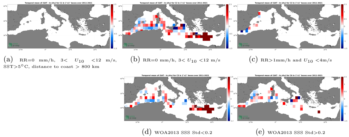
Figure 12: Temporal mean gridded over spatial boxes of size 1^\circ \times 1^\circ of \Delta SSS (SMOS SSS L4 v2 - Daily (BEC) - TSG (CSIC-UTM)) for 5 different subdatasets corresponding to:RR=0 mm/h, 3 < U_{10} < 12 m/s, SST >5^\circ\text{C} , distance to coast > 800 km (a), RR=0 mm/h, 3 < U_{10} < 12 m/s (b), RR >1 mm/h and U_{10} < 4 m/s (c), WOA2013 SSS Std <0.2 (d), WOA2013 SSS Std >0.2 (e).
