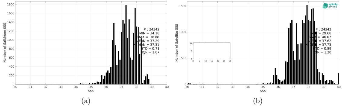
Figure 3: Histograms of SSS from Saildrone (a) and SMOS SSS L4 v2 - Daily (BEC) (b) considering all match-up pairs per bins of 0.1 over the Mediterranean Sea Pi-MEP region and for the full satellite product period.
