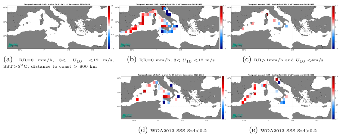
Figure 14: Temporal mean gridded over spatial boxes of size 1^\circ \times 1^\circ of \Delta SSS (SMOS SSS L4 v2 - Daily (BEC) - Saldrone) for 5 different subdatasets corresponding to:RR=0 mm/h, 3 < U_{10} < 12 m/s, SST>5°C, distance to coast > 800 km (a), RR=0 mm/h, 3 < U_{10} < 12 m/s (b), RR.>1mm/h and U_{10} < 4 m/s (c), WOA2013 SSS Std<0.2 (d), WOA2013 SSS Std>0.2 (e).
