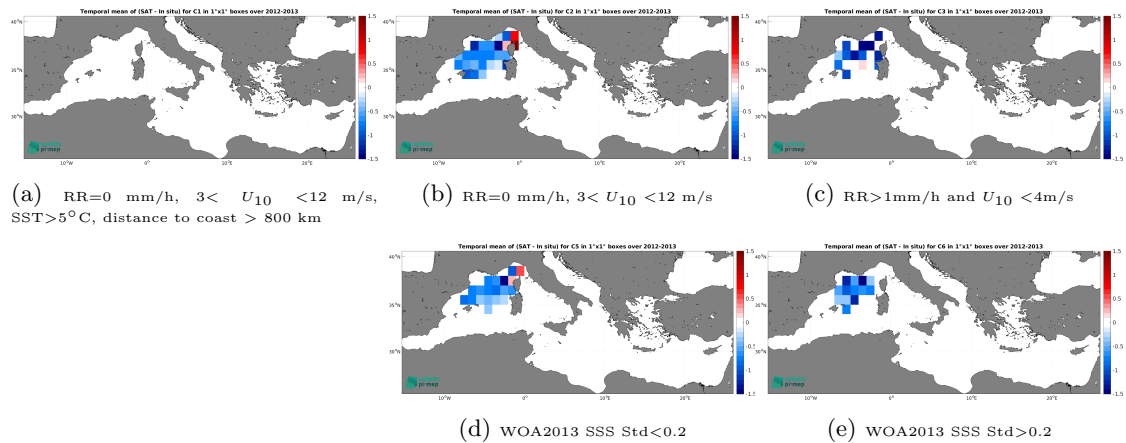
Figure 11: Temporal mean gridded over spatial boxes of size 1^\circ \times 1^\circ of \Delta\text{SSS} (SMOS SSS L4 v2 - Daily (BEC) - Surface drifters) for 5 different subdatasets corresponding to:RR=0 mm/h, 3 < U_{10} < 12 m/s, SST >5^\circ\text{C} , distance to coast > 800 km (a), RR=0 mm/h, 3 < U_{10} < 12 m/s (b), RR >1 mm/h and U_{10} < 4 m/s (c), WOA2013 SSS Std <0.2 (d), WOA2013 SSS Std >0.2 (e).
