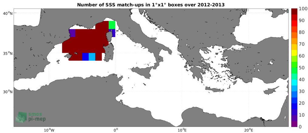
Figure 3: Number of SSS match-ups between Surface drifters SSS and the SMOS SSS L4 v2 - Daily (BEC) SSS product for the Mediterranean Sea Pi-MEP region over 1^\circ \times 1^\circ boxes and for the full satellite product period.
