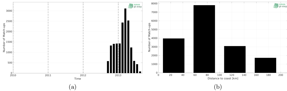
Figure 1: Number of match-ups between Surface drifters and SMOS SSS L4 v2 - Daily (BEC) SSS as a function of time (a) and as function of the distance to coast (b) over the Mediterranean Sea Pi-MEP region and for the full satellite product period.
