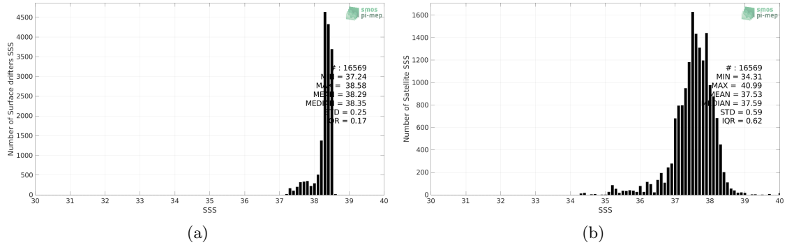
Figure 2: Histograms of SSS from Surface drifters (a) and SMOS SSS L4 v2 - Daily (BEC) (b) considering all match-up pairs per bins of 0.1 over the Mediterranean Sea Pi-MEP region and for the full satellite product period.
